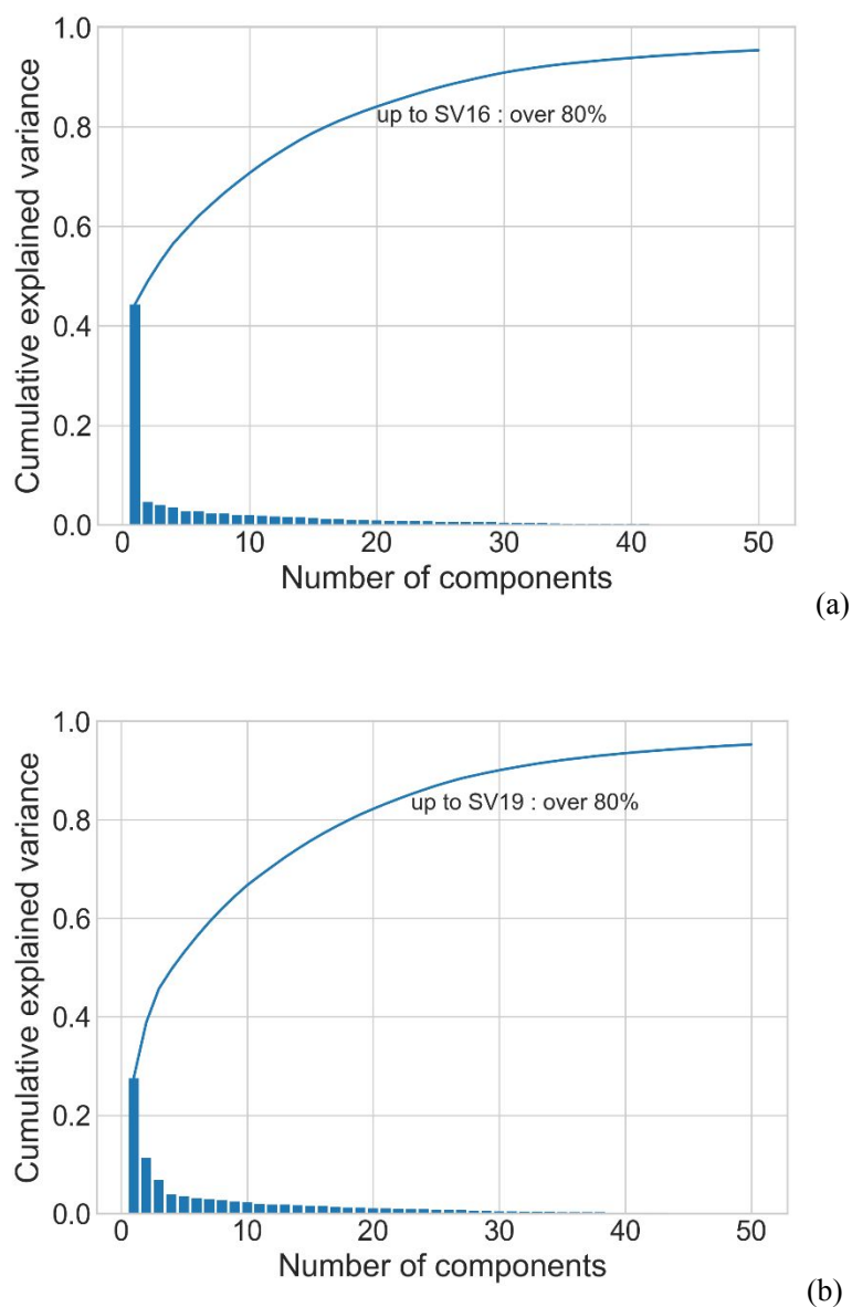
Figure 12. Distributions of eigenvalues in SVD in the presence (a) and absence (b) of the covalent bond to C145. Solid curves represent the cumulative contributions.
