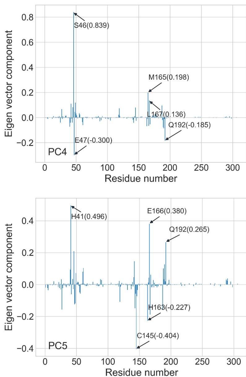
Figure S5. PCA results for stage 2 (30-100 ns) in the case of the absence of the covalent bond between N3 and C145. Following the distribution of the eigenvalues, the residue components for the eigenvectors of PC1-PC5 are illustrated.
