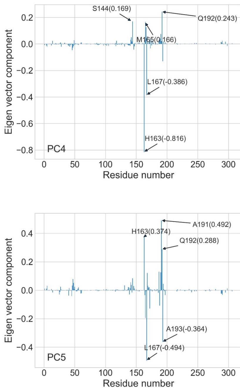
Figure 7. Residue components for the eigenvectors of PC1-PC5 in PCA in the presence of the covalent bond with C145.
