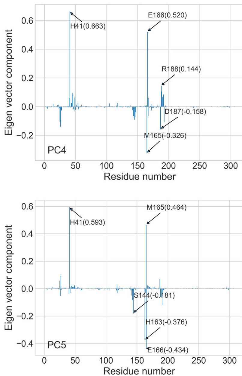
Figure S4. PCA results for stage 1 (0-30 ns) in the case of the absence of the covalent bond between N3 and C145. Following the distribution of the eigenvalues, the residue components for the eigenvectors of PC1-PC5 are illustrated.
