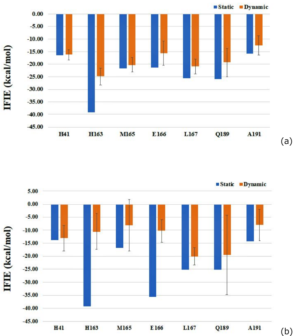
Figure 4. IFIE values of leading residues interacting (larger than -10 kcal/mol of total stabilization) with M^{\text{pro}} in the cases of the presence (a) and absence (b) of the covalent bond between N3 and C145. Blue and orange bars correspond to the single value by “static” structure and the averaged value by a thousand “dynamic” structures, respectively. Vertical line for the latter refers to the standard deviation.
