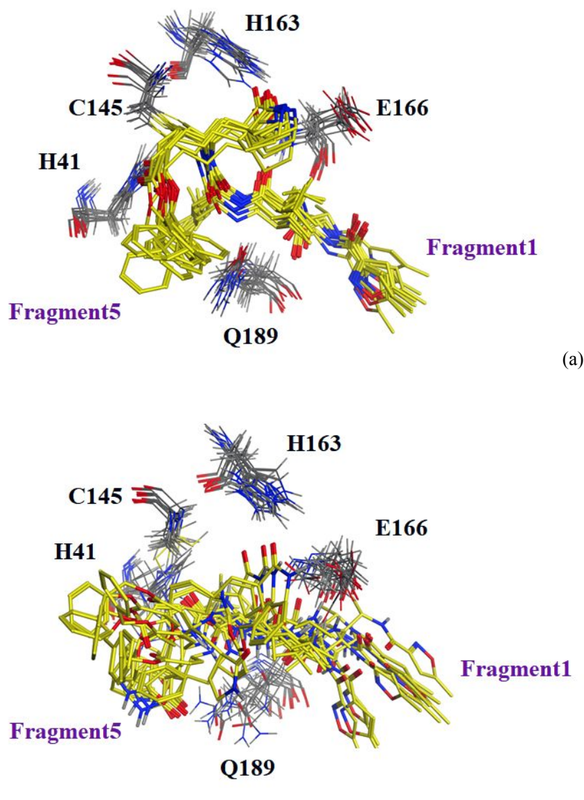
Figure 3. Superimposed view of snapshots from the 100 ns MD trajectory sampled with 10 ns intervals for the N3 ligand and crucial residues in pharmacophore. (a) The N3 ligand which is covalently bonded to C145 is depicted in yellow color. (b) The N3 ligand depicted in yellow is not covalently bonded to C145.
