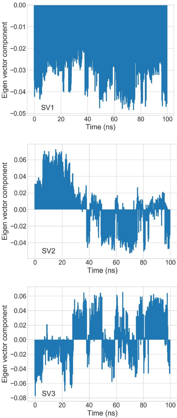
Figure 11. Temporal components (U) for the eigenvectors of SV1-SV3 in SVD in the absence of the covalent bond to C145.
