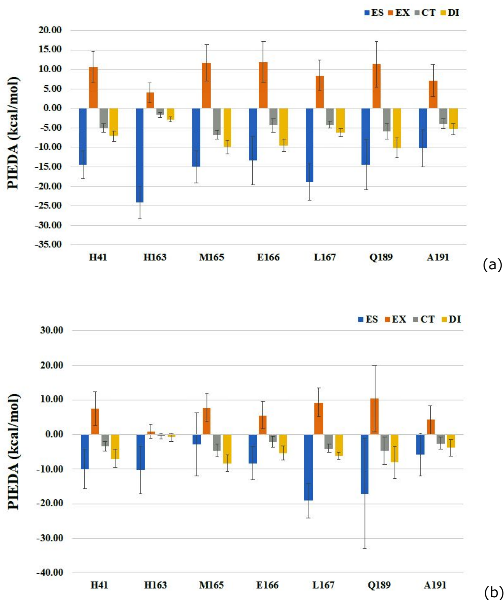
Figure 5. Averaged PIEDA values of crucial residues interacting (more than -10 kcal/mol of total stabilization) with M pro over a thousand “dynamic” structures in the cases of the presence (a) and absence (b) of the covalent bond between N3 and C145. Blue, orange, gray and yellow bars correspond to ES, EX, CT and DI terms, respectively. Vertical line refers to the standard deviation.
