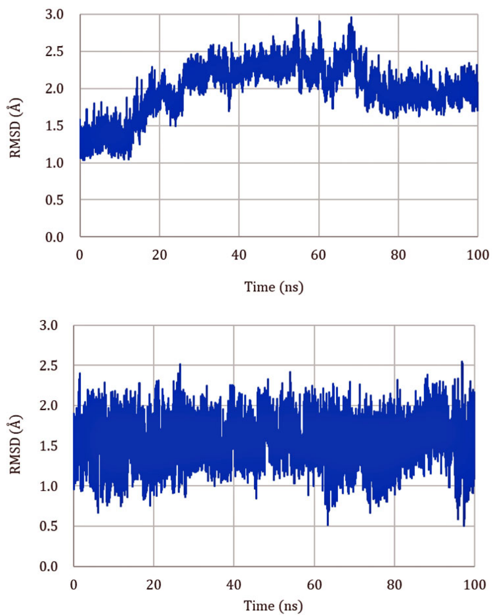
Figure S2. RMSDs for 100 ns MD in the presence of the covalent bond between N3 ligand and C145 residue of M Pro . Upper panel: C \alpha atoms in M Pro . Lower panel: C and N atoms in N3.
