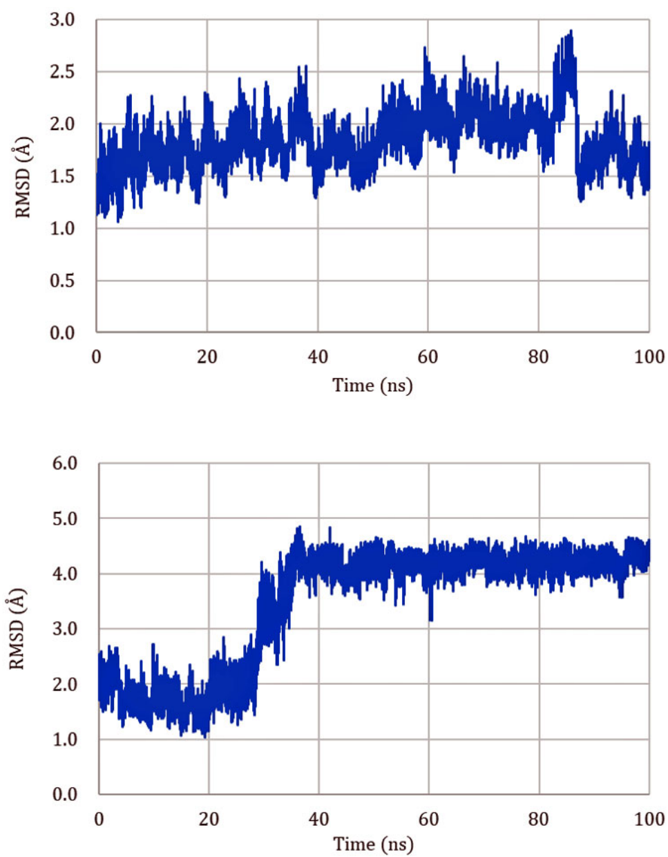
Figure S3. RMSDs for 100 ns MD in the absence of the covalent bond between N3 ligand and C145 residue of M pro . Upper panel: C α atoms in M pro . Lower panel: C and N atoms in N3.
