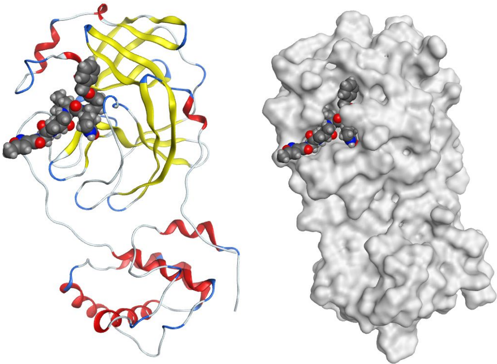
Figure 1. Structure of M^{\text{pro}} -N3 complex (PDB entry: 6LU7) by two ways in which M^{\text{pro}} is depicted by ribbon (left) and molecular surface (right) representations. The N3 ligand is depicted by the sphere representation.
