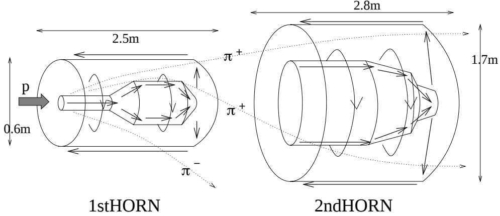
Figure 2.5: Target and magnetic horn. The target is an aluminum rod. Both horns only focus positive pions.
