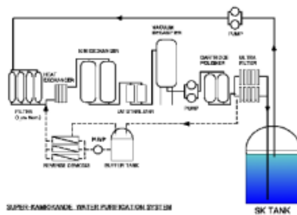
Figure 2.14: SK water purification system.
