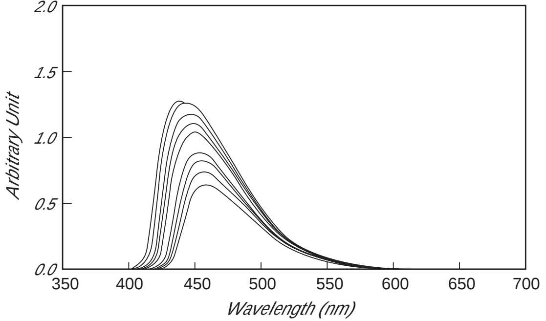
Figure 3.3: SCSF-78M (version 11) light wavelength. The eight lines correspond to measurement at 20cm, 40cm,... 160cm from the entrance point of the light.
