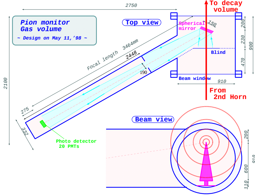
Figure 2.7: Pion monitor.
