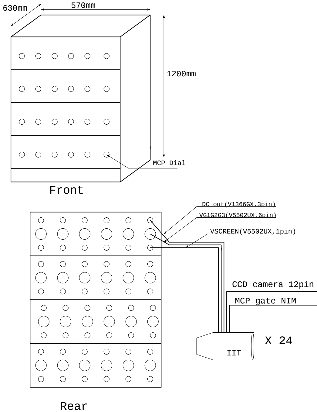
Figure 3.15: HV supplier for 24 IITs.
