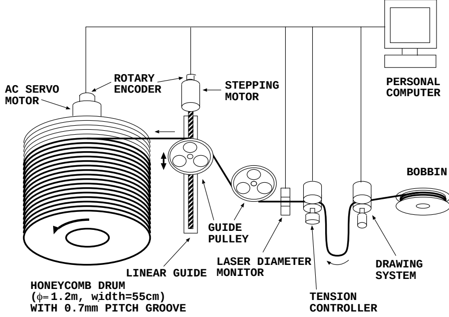
Figure 3.6: SciFi sheet spooling machine.
