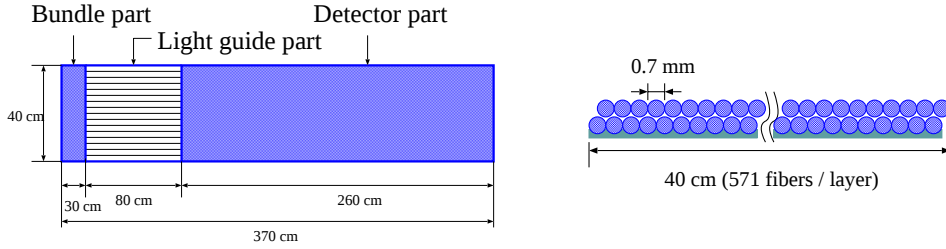
Figure 3.8: Top view (left) and cross section (right) of SciFi sheet.
