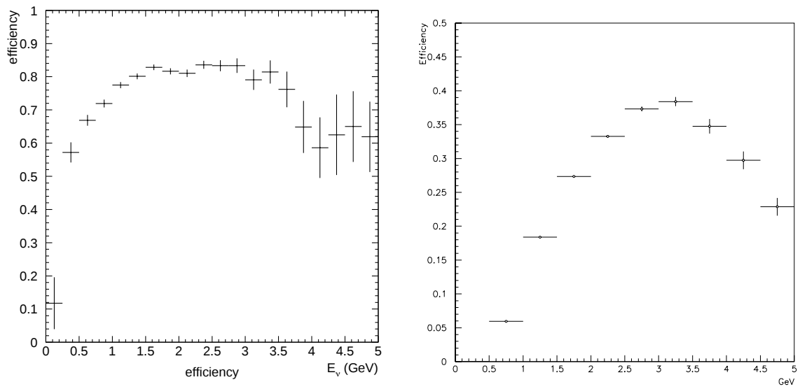
Figure 6.6: SK/SciFi detection efficiency as a function of neutrino energy (GeV).
