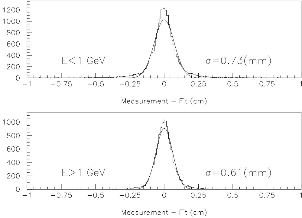
Figure 5.6: Hit residual distributions using neutrino beam data. The curve is a single Gaussian fit to the data with \sigma = 0.73\text{mm} ( 0.61\text{mm} ) for muon energy E_\mu < 1\text{GeV} ( E_\mu > 1\text{GeV} ).
