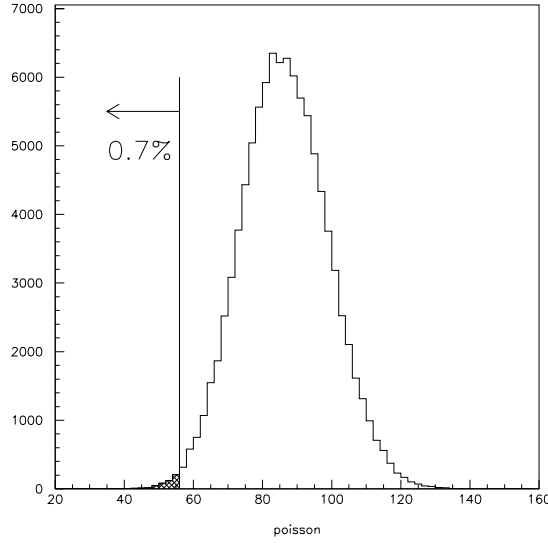
Figure 9.1: A poisson distribution ( \mu_0 = 85.9 , and \Delta\mu = 8.5 ) smeared by Gaussian. By a 10^6 times test, the probability is 0.7% for the observation of 56 events.
