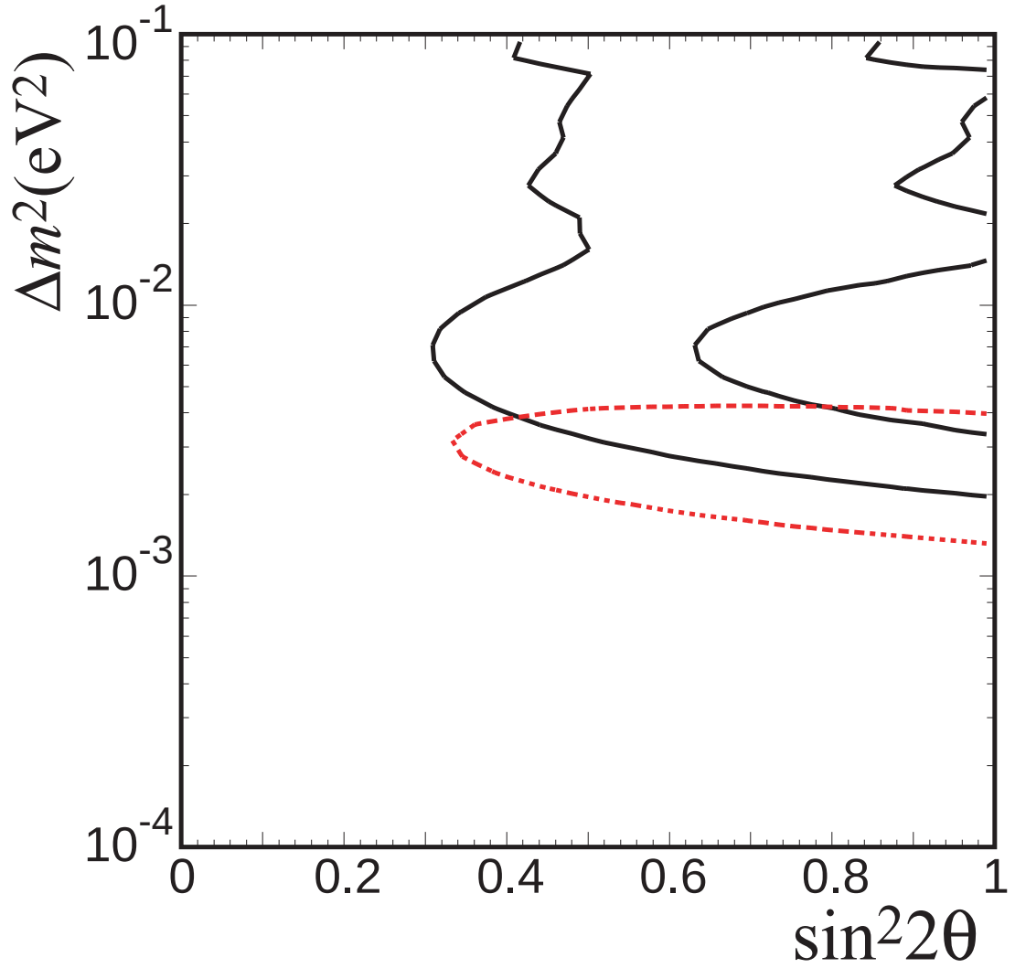
Figure 9.4: Allowed regions (68% C.L.) of oscillation parameters given by normalization only (solid) and shape only (dashed). The inside of the two solid lines and the right side of the dashed curve are the allowed regions.
