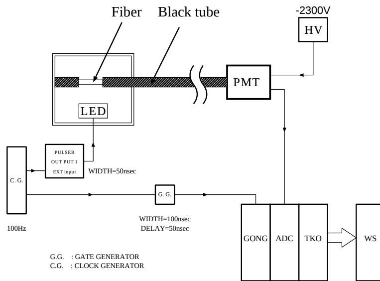
Figure 4.3: Setup of LED calibration.
