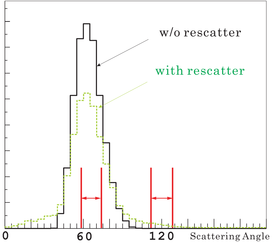
Figure 4.2: Scattering angle distributions for \nu_e MC with and without final state interaction. Alanakyan et al. measured proton number ratio between the scattered angle 120 \pm 8^\circ and 66 \pm 8^\circ .
