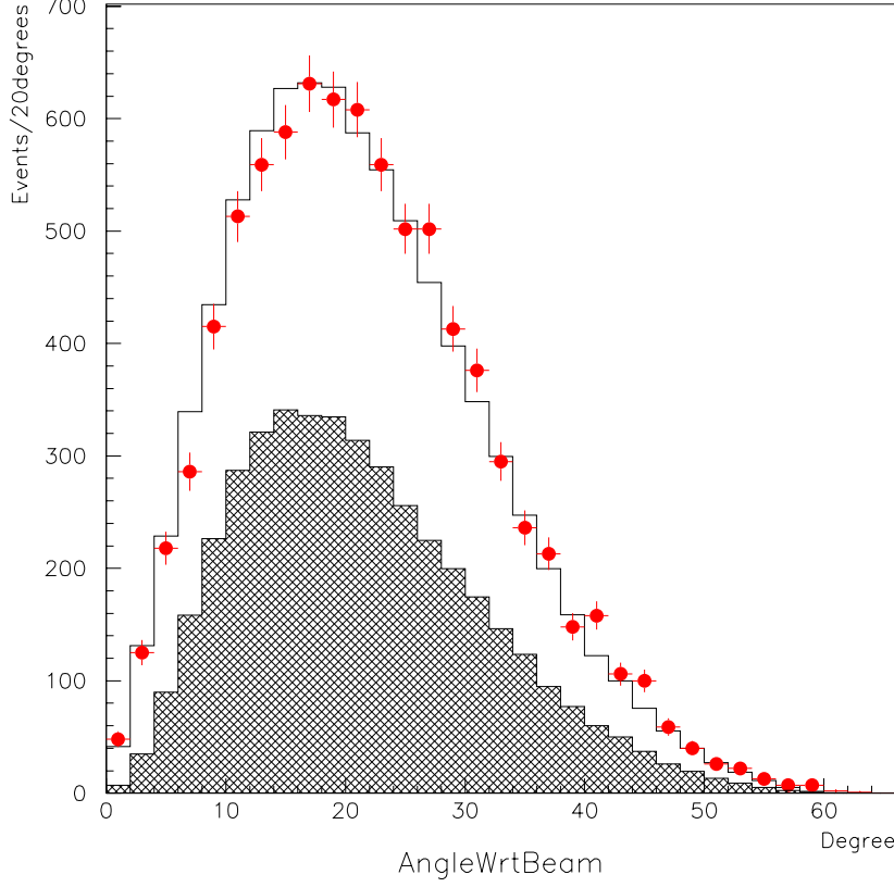
Figure 7.2: \theta_\mu distribution of MRD events.
