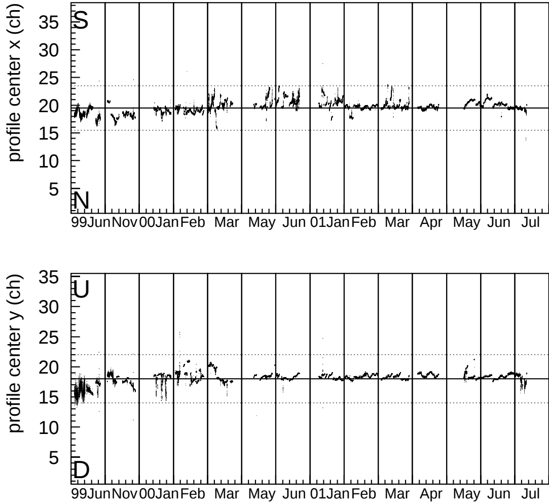
Figure 6.2: Neutrino beam direction stability measured by the muon monitor (ionization chamber). The top figure shows the horizontal profile, the bottom figure the vertical. The X-axis is months; The Y-axis is the readout channel. The solid line points in the direction of the far detector. The broken lines correspond to within \pm 1\text{mrad} . difference from this direction.
