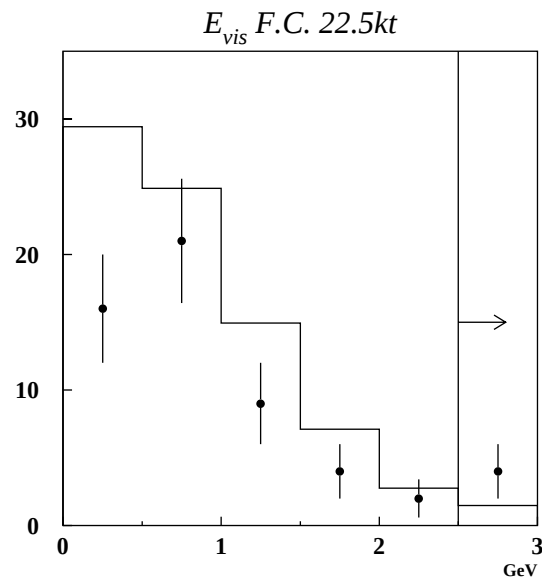
Figure 8.3: Visible energy distribution of SK events.
