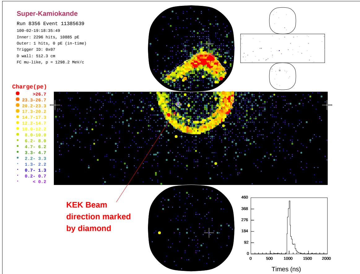
Figure 8.2: Typical neutrino event at SK. The observed charge for each PMT is indicated by the color scale. The black map shows the ID PMTs. The upper white figure shows the OD PMTs. The lower right figure shows the timing distribution in nsec.
