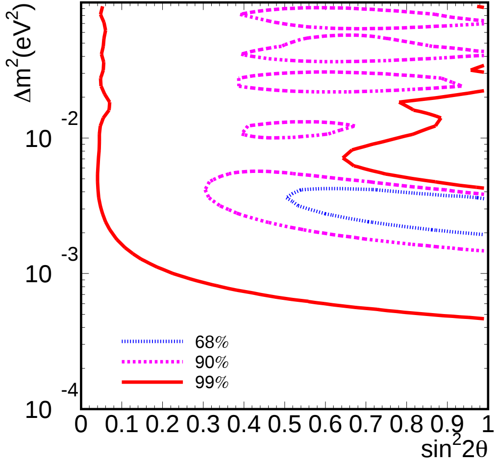
Figure 9.3: Allowed regions of oscillation parameters. The insides of the two solid lines are 99% C.L. The right side of dashed line and the insides of the distorted circles of dashed line are the 90% C.L. The right side of dotted line is 68% C.L.
