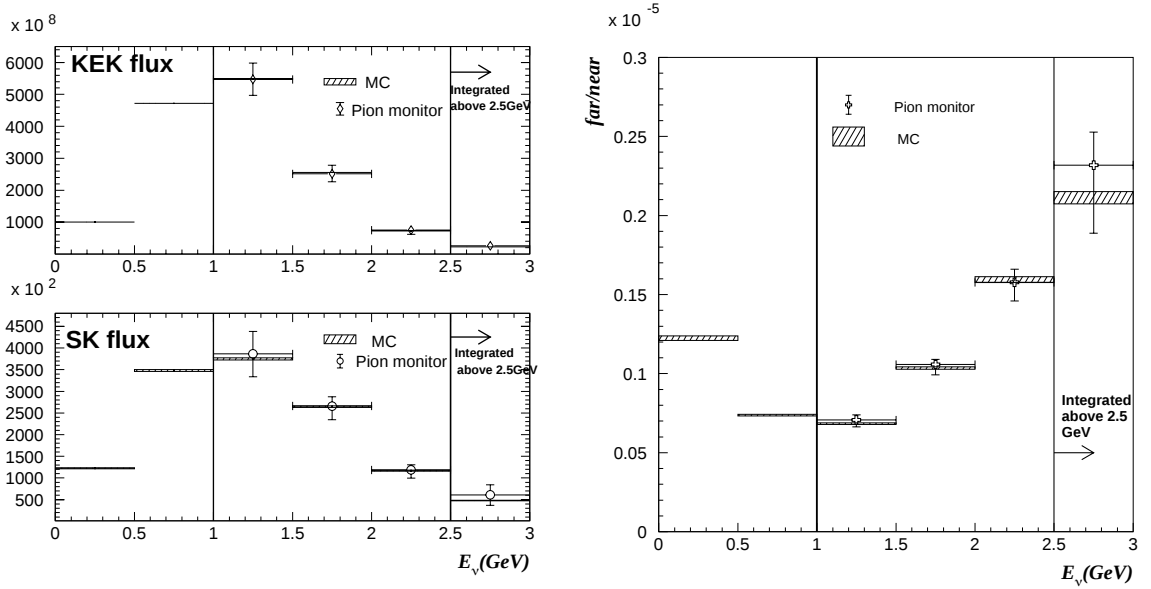
Figure 6.5: Neutrino spectrum (left) and R_{SK/Near} (right) estimated by pion monitor. MC results (the Cho model) are overlaid. (November configuration)
