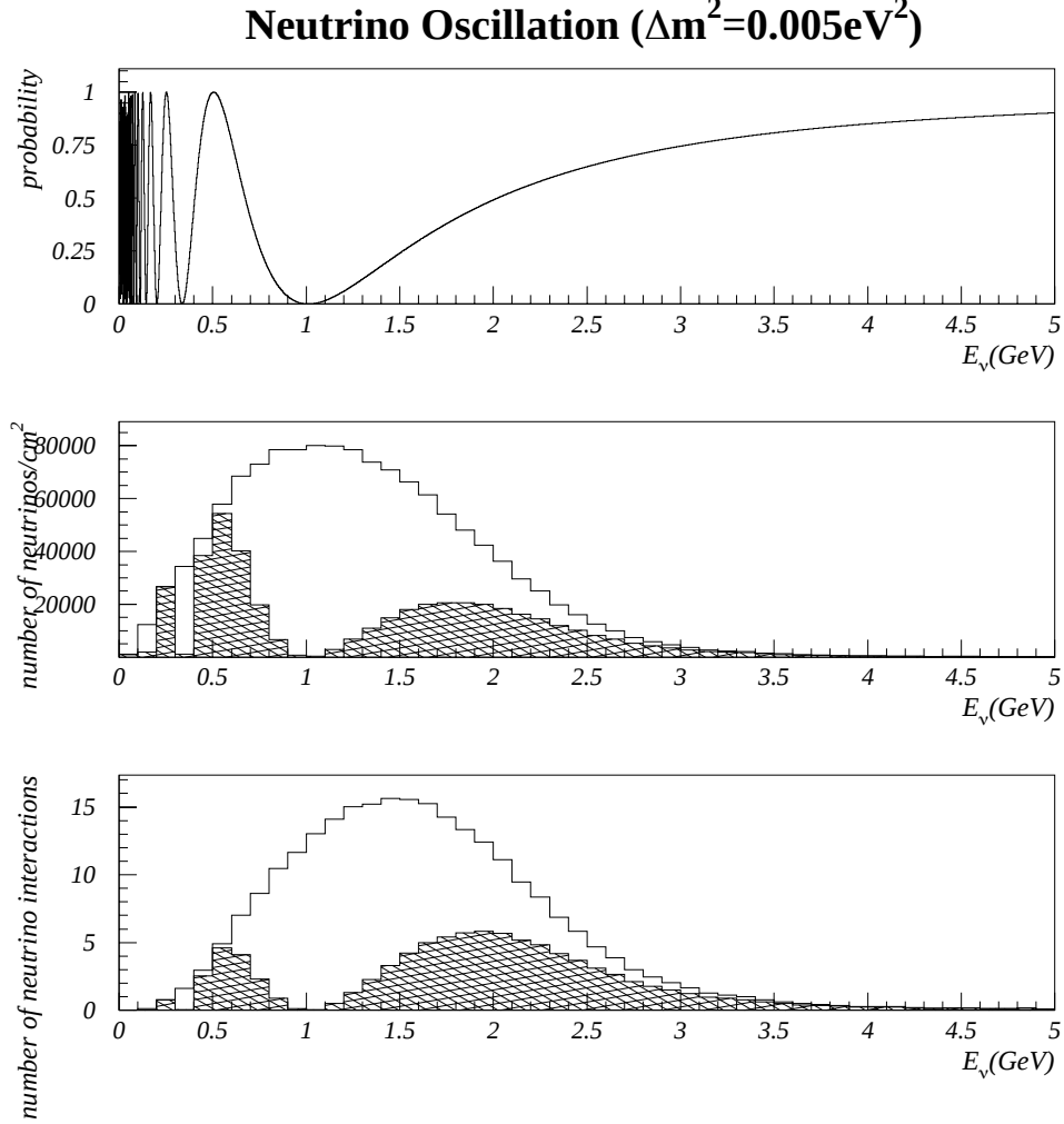
Figure 1.2: Neutrino energy spectrum distortion in K2K in the case of the oscillation at ( \Delta m^2 = 0.005 \text{eV}^2 , \sin^2 2\theta = 1 ). The top figure shows the probability of neutrino oscillation as a function of energy. The middle figure shows the neutrino flux at SK. The histogram shows the expected neutrino flux by MC [units are “number of neutrinos/cm 2 /10 20 POT(Protons On Target)”]. The hatched area is the expected flux times the oscillation probability. The bottom figure shows the neutrino flux times the total cross section of neutrino interaction with water, which corresponds to the expected number of events at SK.
