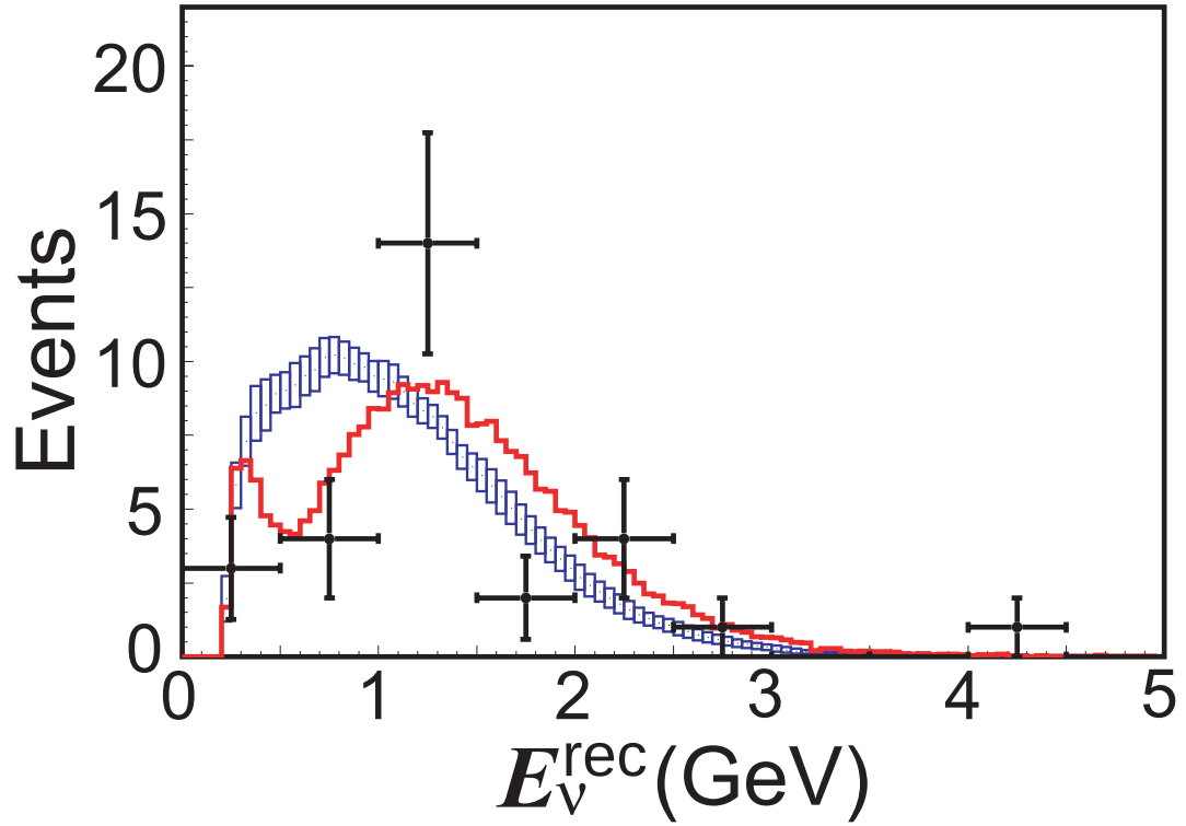
Figure 9.2: The reconstructed E_\nu distribution. Dots are observations, the box histogram is the expected spectrum without oscillations. The height of the boxes are the systematic error sizes. The open histogram is the best fit spectrum. The area of both histograms is normalized to the observations.
