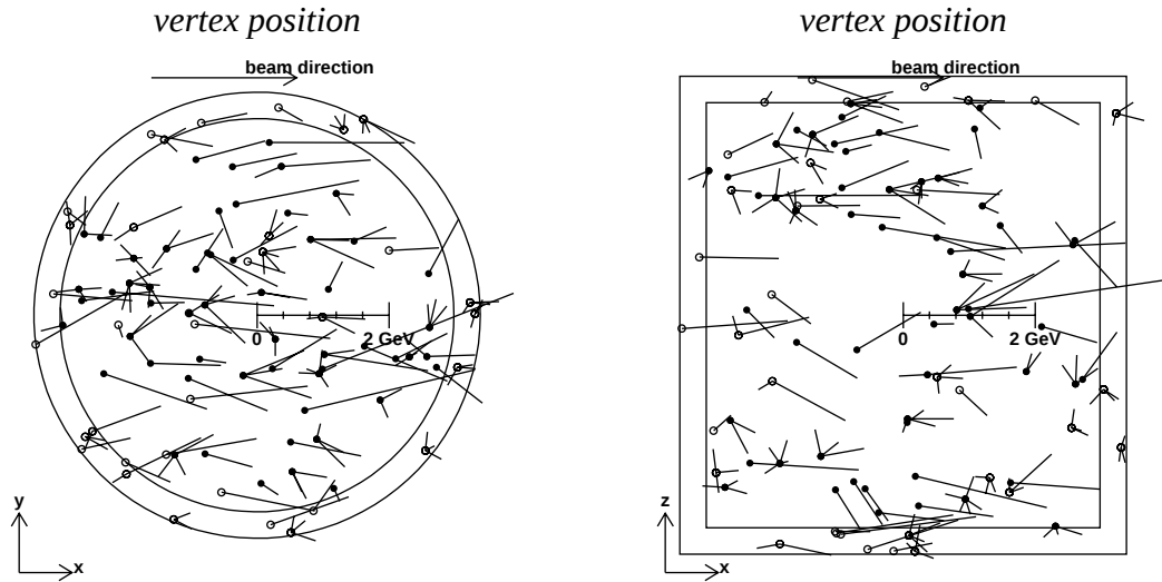
Figure 8.6: Reconstructed vertex distribution of SK events. The left figure shows the top view and the right figure shows the side view with respect to beam direction. The outer circle and box represent the inner detector wall. The inner circle and box represents the fiducial volume boundary. Each circle point shows a reconstructed vertex position. Its line shows the reconstructed particle momentum along the Čerenkov ring. Open circles are events whose vertices fall outside the fiducial volume. Closed circles are events whose vertices fall inside the fiducial volume (FC 56 events after D_{Wall} cut).
