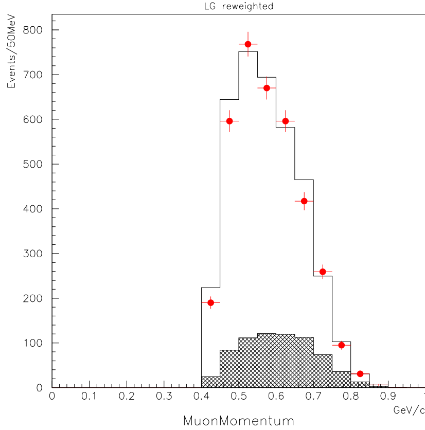
Figure 7.5: P_\mu distribution of LG events.
