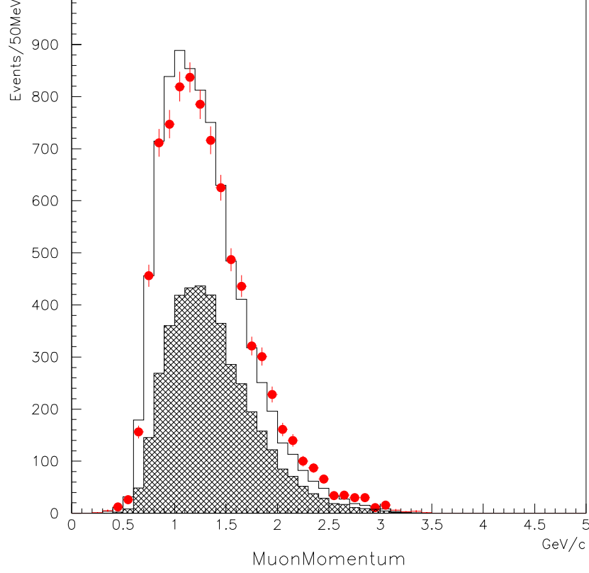
Figure 7.1: P_\mu distribution of MRD events.
