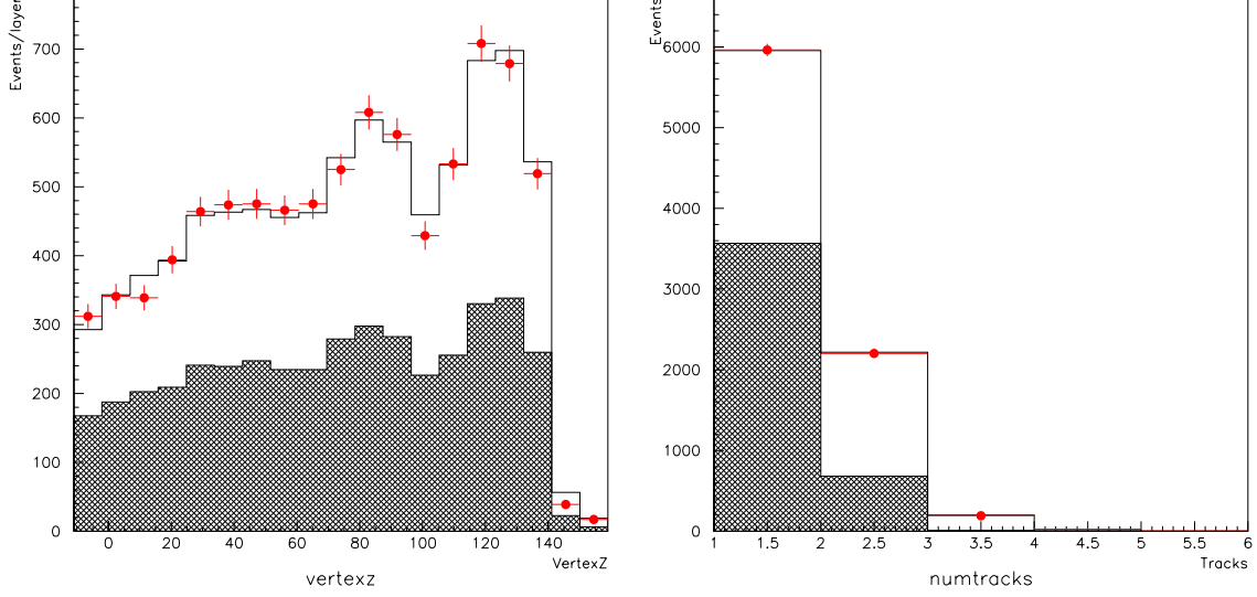
Figure 7.4: Reconstructed event vertices distribution for Z direction (left) and distribution of number of tracks (right). Both plots show MRD sample.
