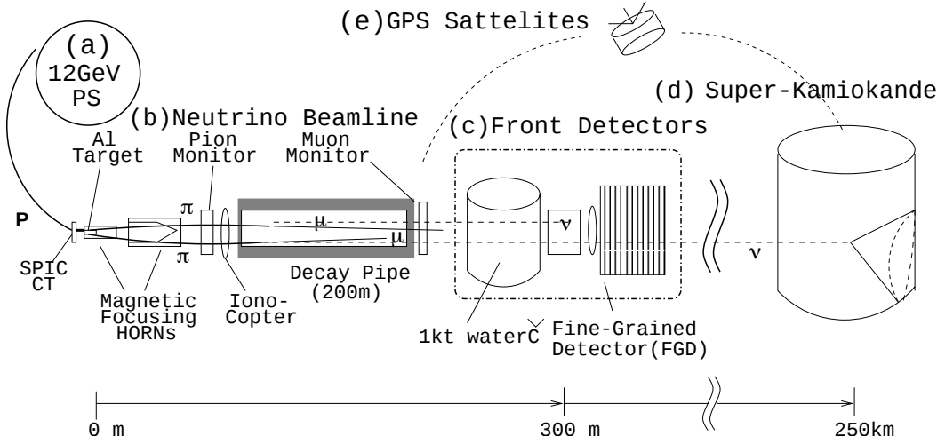
Figure 2.1: Schematic overview of K2K experiment.
