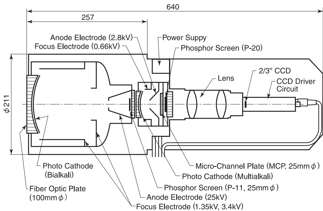
Figure 3.12: IIT-CCD chain.
