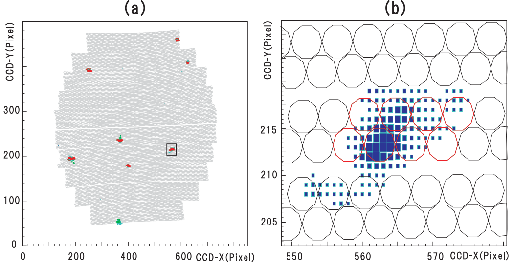
Figure 5.1: (a) A typical CCD image of a cosmic-ray event. (b) This expanded view of (a) shows a typical SciFi hit. Circles inside the figures represent the coordinates of the SciFi in the CCD view. The size of hit pixel is proportional to the brightness in the ADC. Hit fibers are represented by the thick circles. A SciFi hit is defined as a cluster of neighboring hit fibers.
