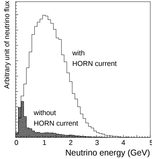
Figure 2.6: Estimated neutrino flux with horn current 0kA and 250kA (simulation). The hatched and white areas correspond to 0kA and 250kA, respectively. 250kA horn current focuses neutrinos 22 times greater than at 0kA.
