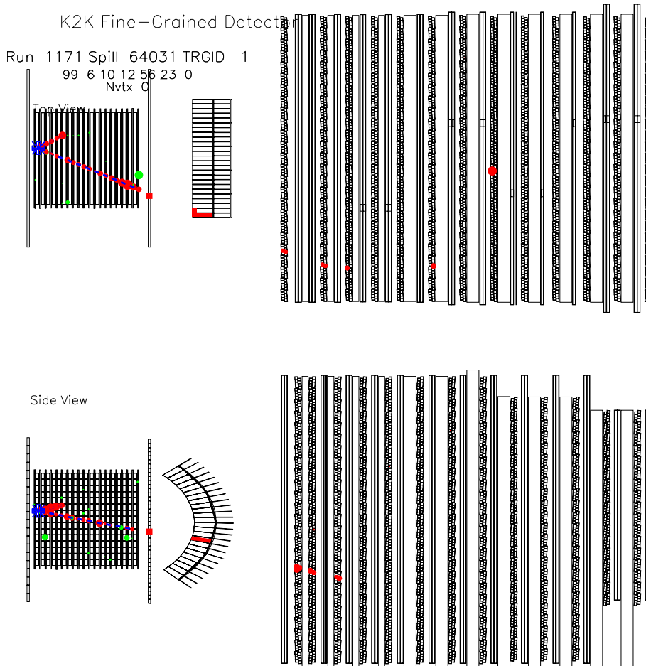
Figure 5.2: Example of a SciFi two-track MRD event. The upper figure is the top view, the lower figure the side view.
