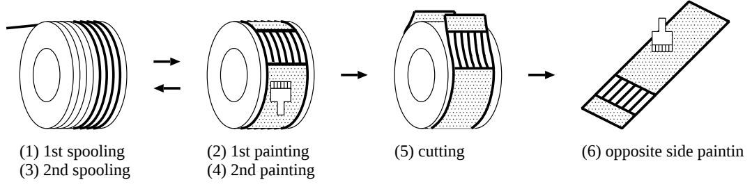
Figure 3.7: SciFi sheet spooling process.
