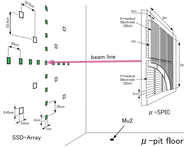
Figure 2.9: Muon monitors.
