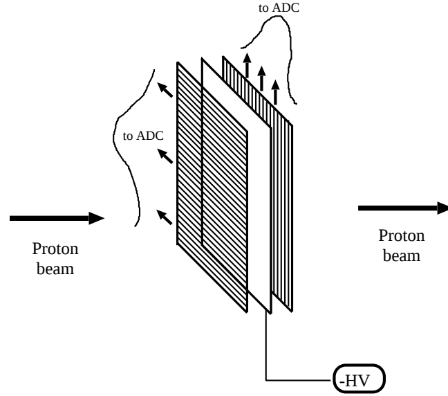
Figure 2.4: Schematic view of a SPIC.
