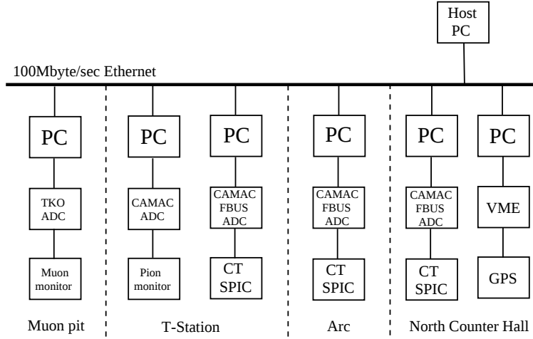
Figure 2.10: Beam line DAQ.
