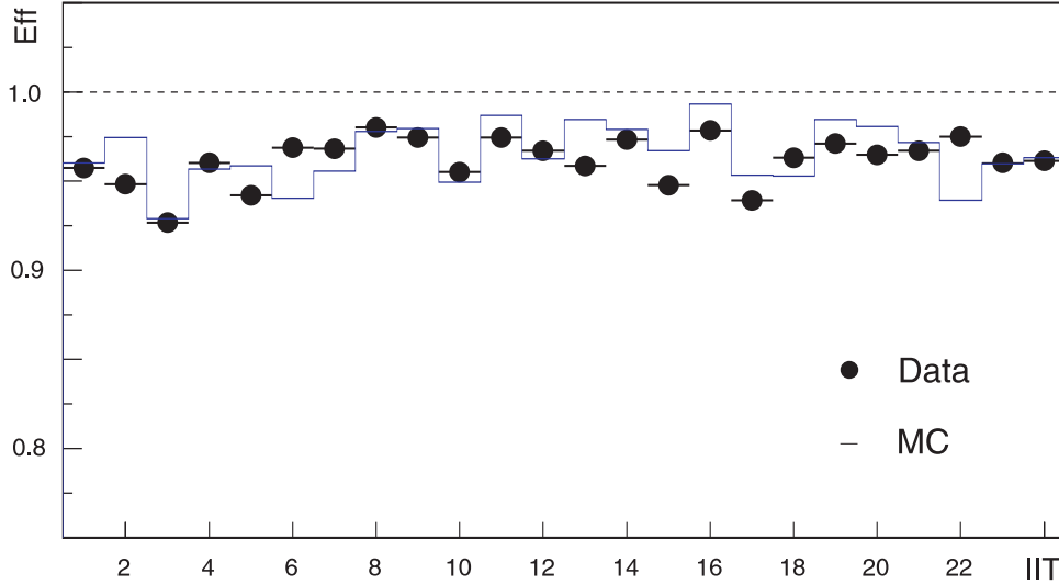
Figure 5.3: Hit finding efficiency of 24IITs.
