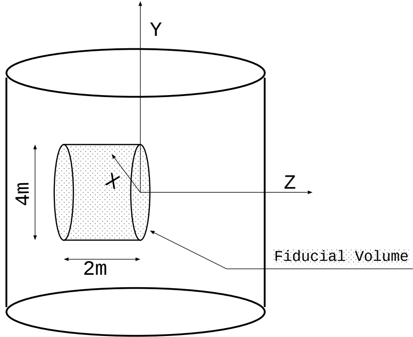
Figure 7.10: Definition of the 25-ton fiducial volume at the 1kt Čerenkov detector.
