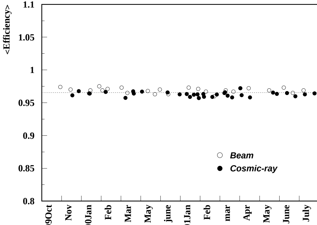
Figure 5.4: Stability of hit finding efficiency from Nov '99 to Jul '01.
