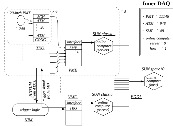
Figure 2.15: The data acquisition system for the inner detector.
