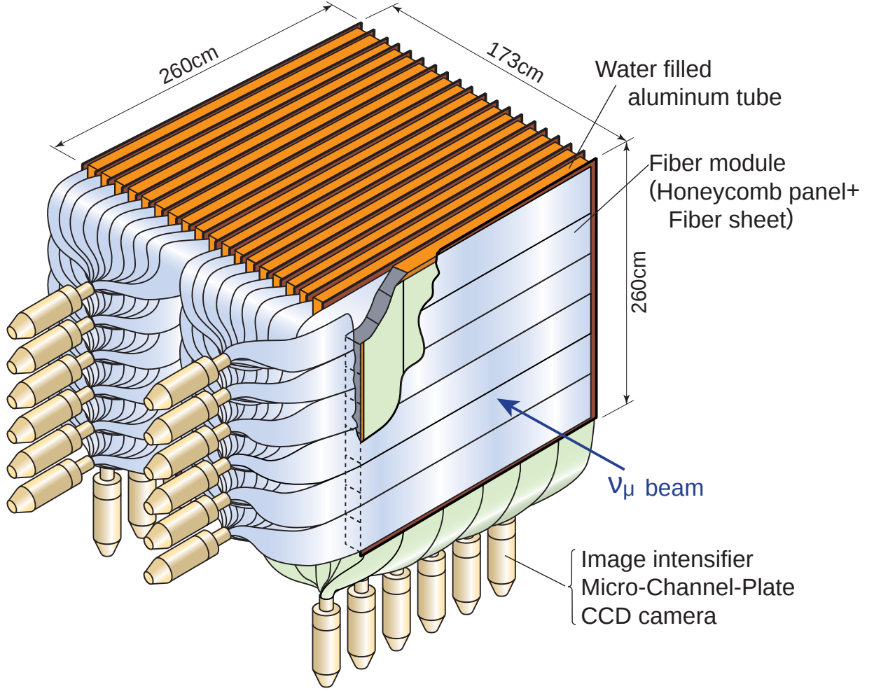
Figure 3.1: Overview of the SciFi detector.
