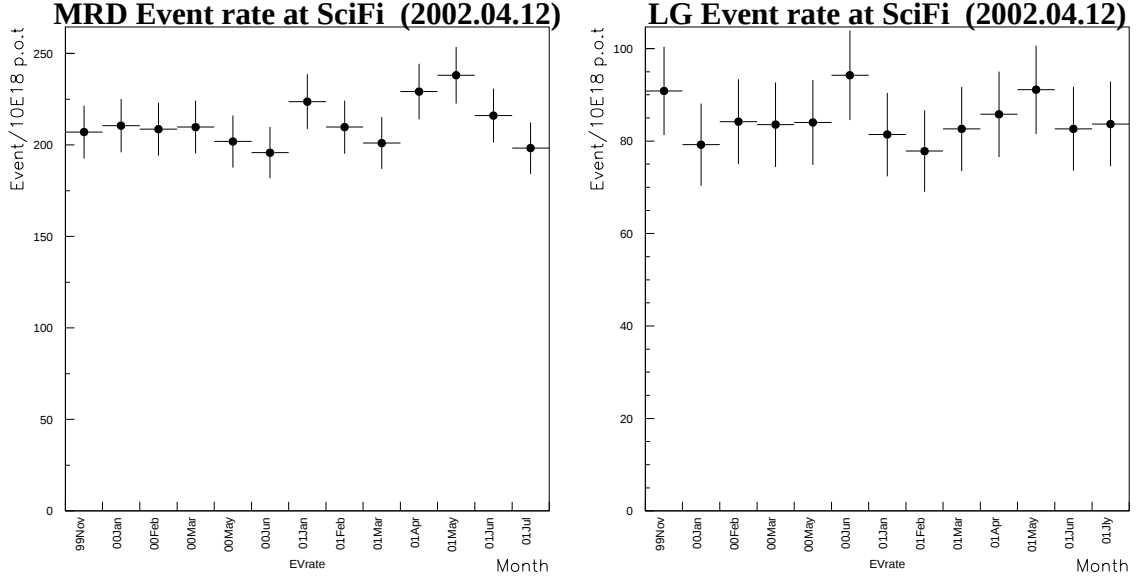
Figure 6.4: SciFi MRD and LG stopping event rate per month normalized by POT_{SciFi} .
