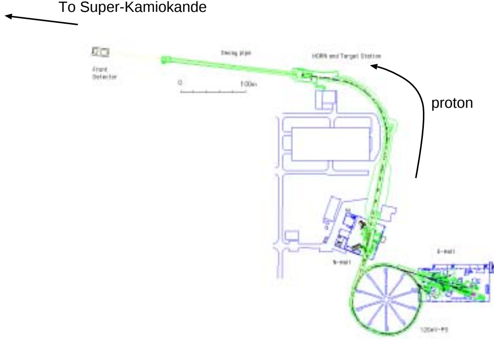
Figure 2.3: Proton beam line.
