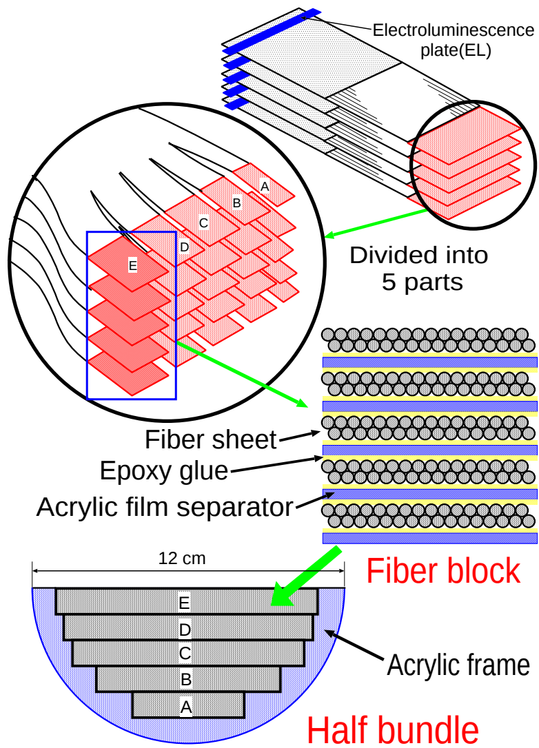
Figure 3.10: How SciFi sheets are bundled.
