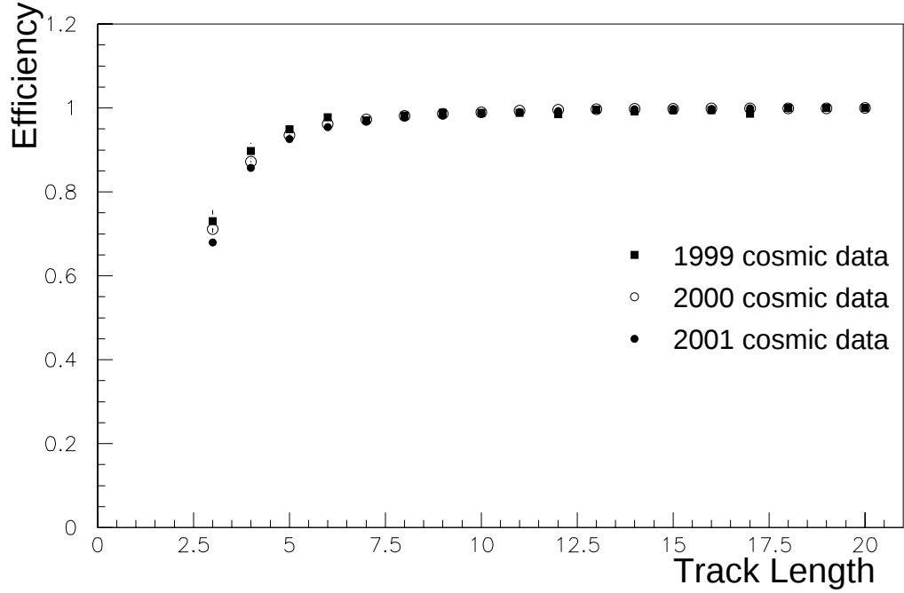
Figure 5.5: Track finding efficiency as a function of the track length. Efficiency is \sim 70\% ( \sim 87\% ) in a track length of the three (four) SciFi layers and approaches 100% in longer tracks.
