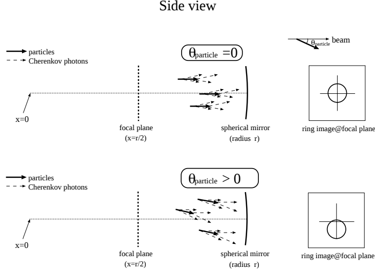
Figure 2.8: Pion monitor measures the angle and momentum of pions.
