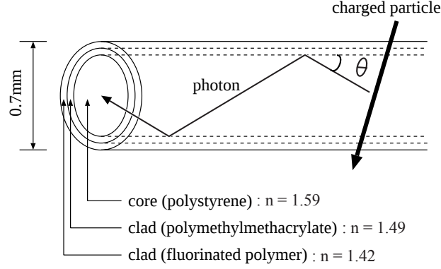
Figure 3.2: Scintillating fiber SCSF-78M (multi-cladding type).
