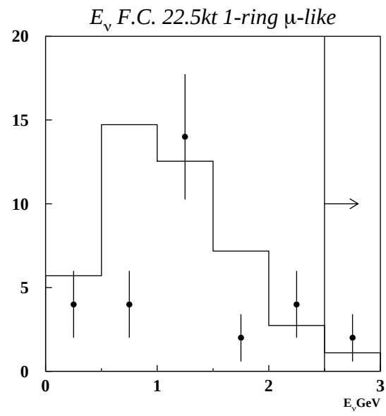
Figure 8.5: Reconstructed neutrino energy distribution of SK events.
