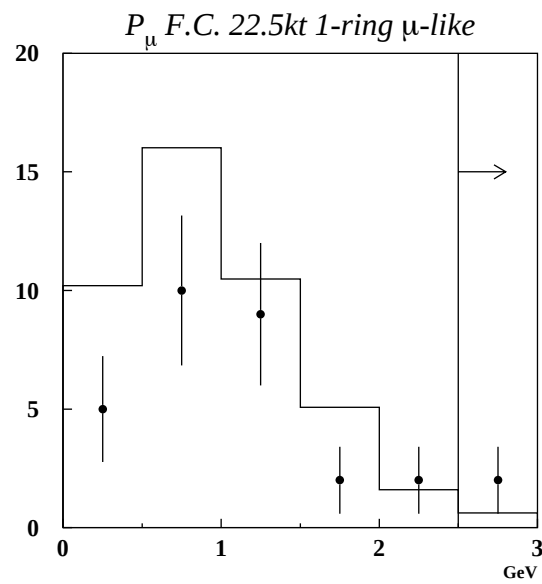
Figure 8.4: Muon momentum distribution of SK events.
