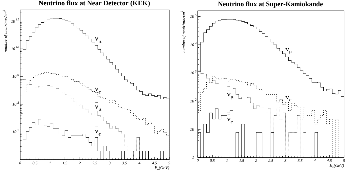
Figure 4.1: Neutrino flux calculated by beam simulation. The hadron production model selected is the Cho model. Left figure: Neutrino flux at KEK. Right figure: Neutrino flux at SK.
