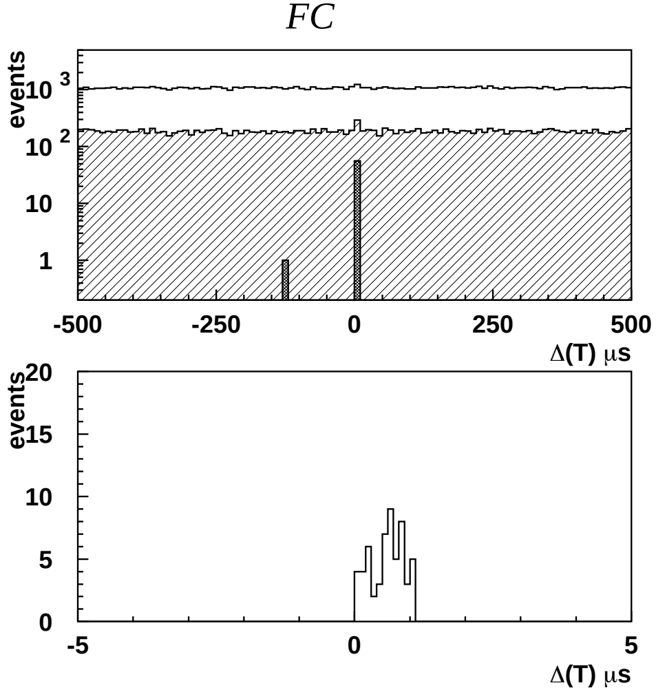
Figure 8.1: Time difference distribution of HE (High Energy) triggered events after decay electron cut (solid line), total photo-electron cut (light hatch), and selected events inside fiducial volume (dark hatch). The upper figure is at \pm 500 \mu\text{sec.} , the lower figure at \pm 5 \mu\text{sec.} A clear peak can be seen within 1.1 \mu\text{sec.} of beam spill width and \pm 0.2 \mu\text{sec.} of GPS precision.
