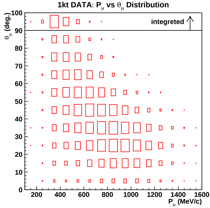
Figure 7.11: Two-dimensional distributions of muon momentum vs. production angle with respect to the beam direction in the 1kt detector.
