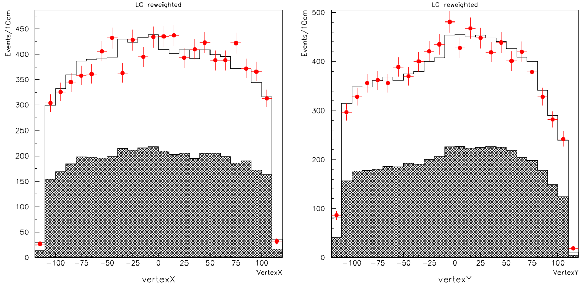
Figure 7.7: Reconstructed LG-event vertices distribution for X (left), Y (right).
