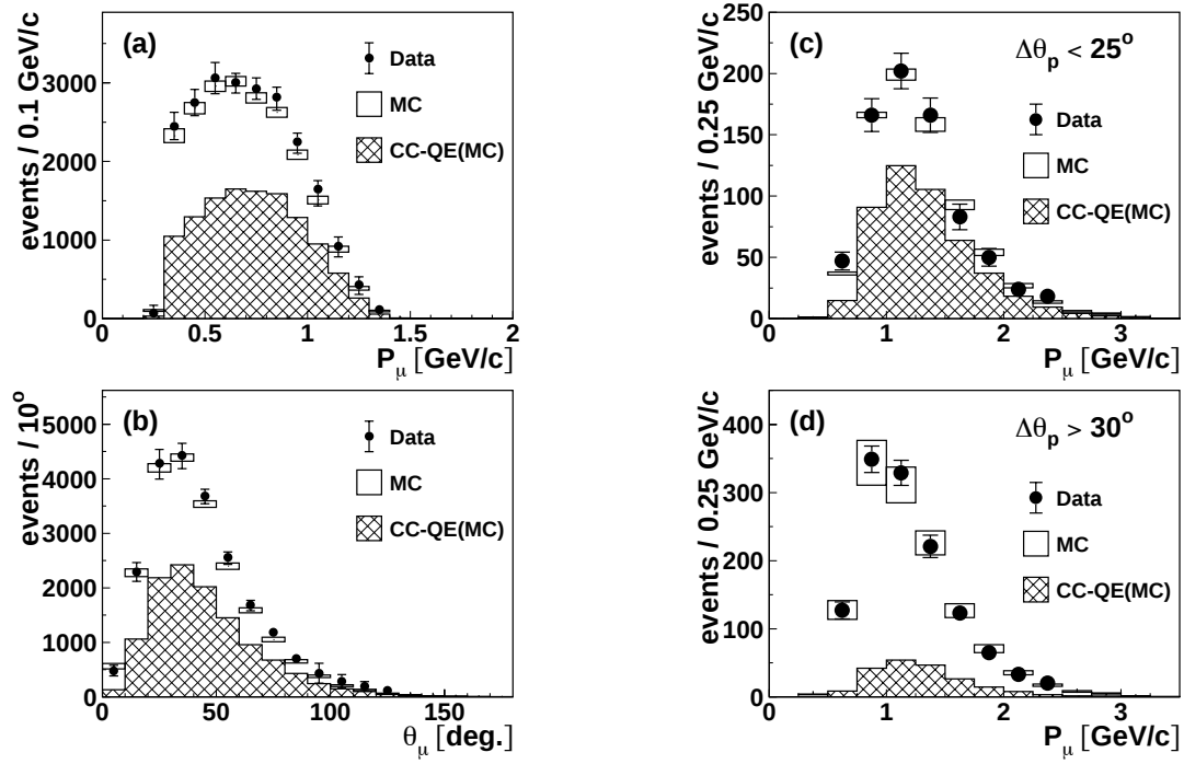
Figure 7.12: (a) The muon momentum distribution of the 1kt detector one-ring \mu samples, (b) the angular distribution of the 1kt one-ring \mu samples, (c) the muon momentum distribution of the SciFi QE samples, and (d) of the SciFi non-QE samples, The dots are data and the boxes are MC simulation with best fit parameters. The hatched histograms are the CCQE events estimated by the MC simulation.
