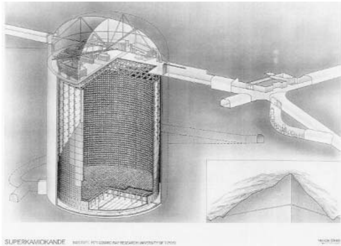
Figure 2.13: Far detector Super Kamiokande.
