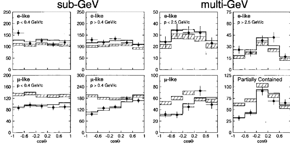
Figure 1.1: The zenith angle distribution of \mu -like and e-like events. Observed neutrino events in SK (cross) and simulation assuming oscillation (line) and no oscillation (hatched box). The distribution is well explained by \nu_\mu \rightarrow \nu_\tau neutrino oscillation where the parameter is \Delta m^2 = 3.2 \times 10^{-3} \text{eV}^2 , \sin^2 2\theta = 1 . "Sub-GeV (Multi-GeV)" indicates events in which visible energy is less (more) than 1.33 GeV.
