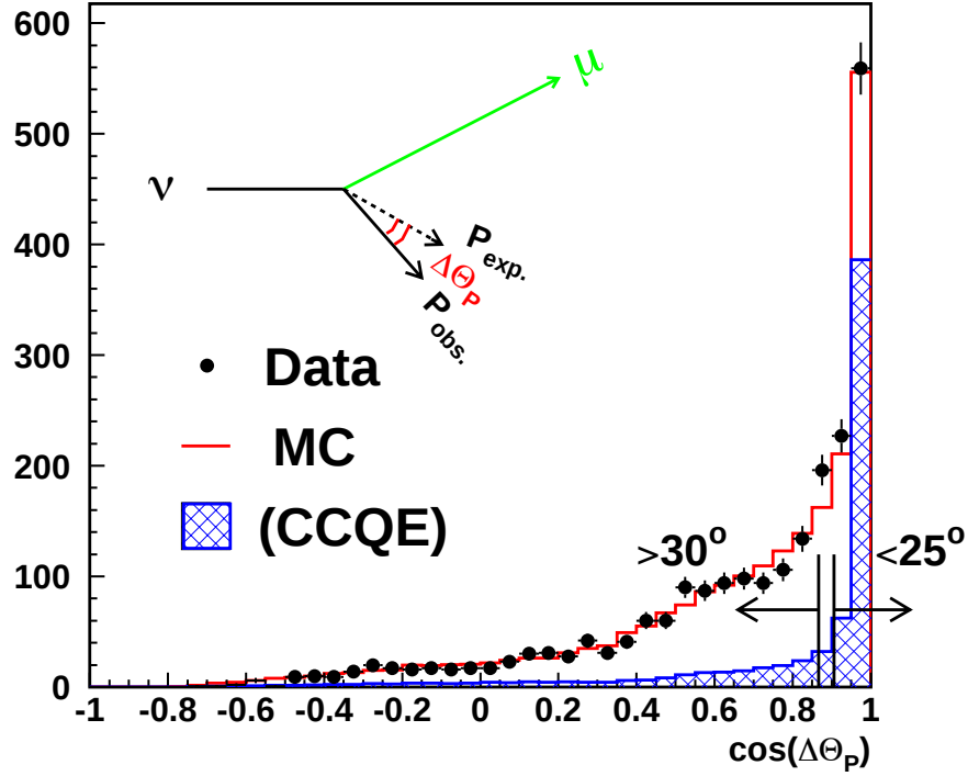
Figure 7.9: \cos \Delta\theta distribution for all two-track MRD events. The hatched area shows MC CCQE events. The diagram shows the definition of \Delta\theta .
