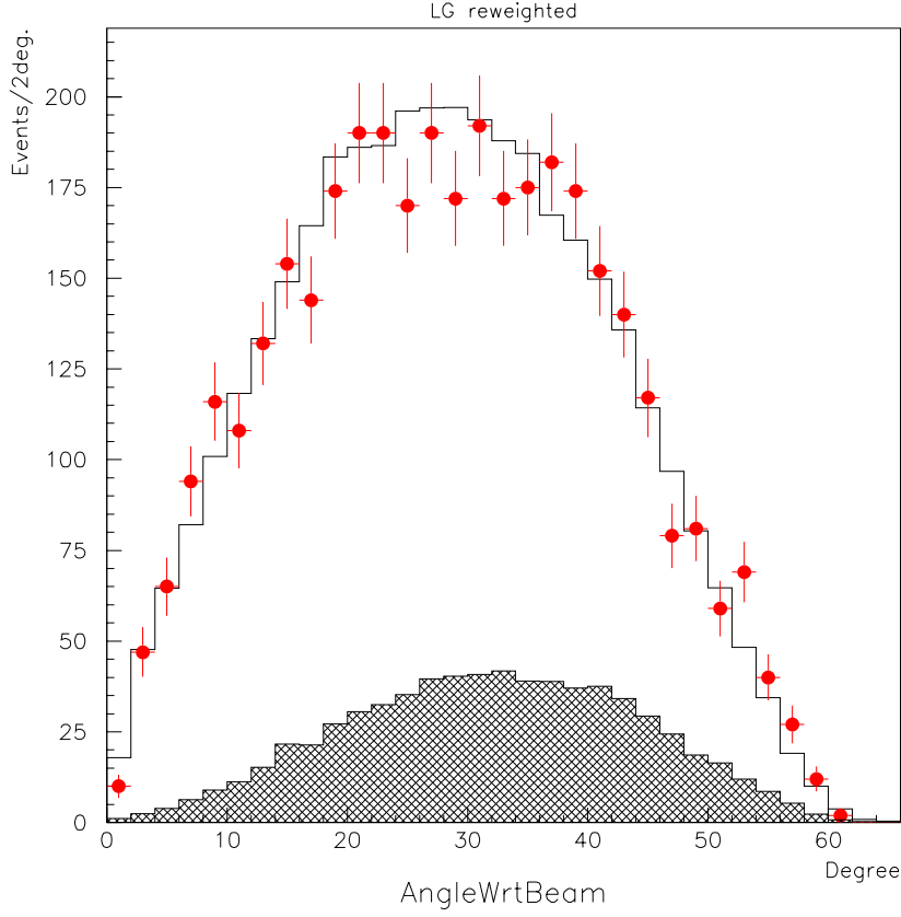
Figure 7.6: \theta_\mu distribution of LG events.
