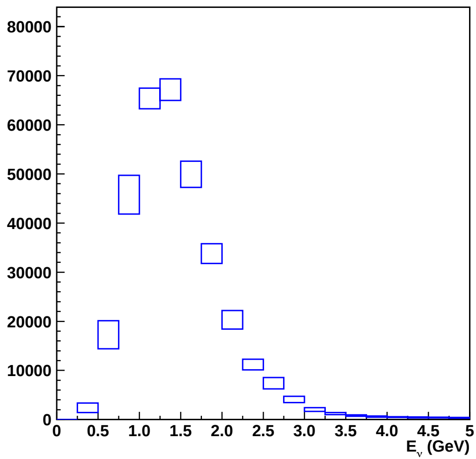
Figure 7.13: Measured neutrino spectrum at near detector.
