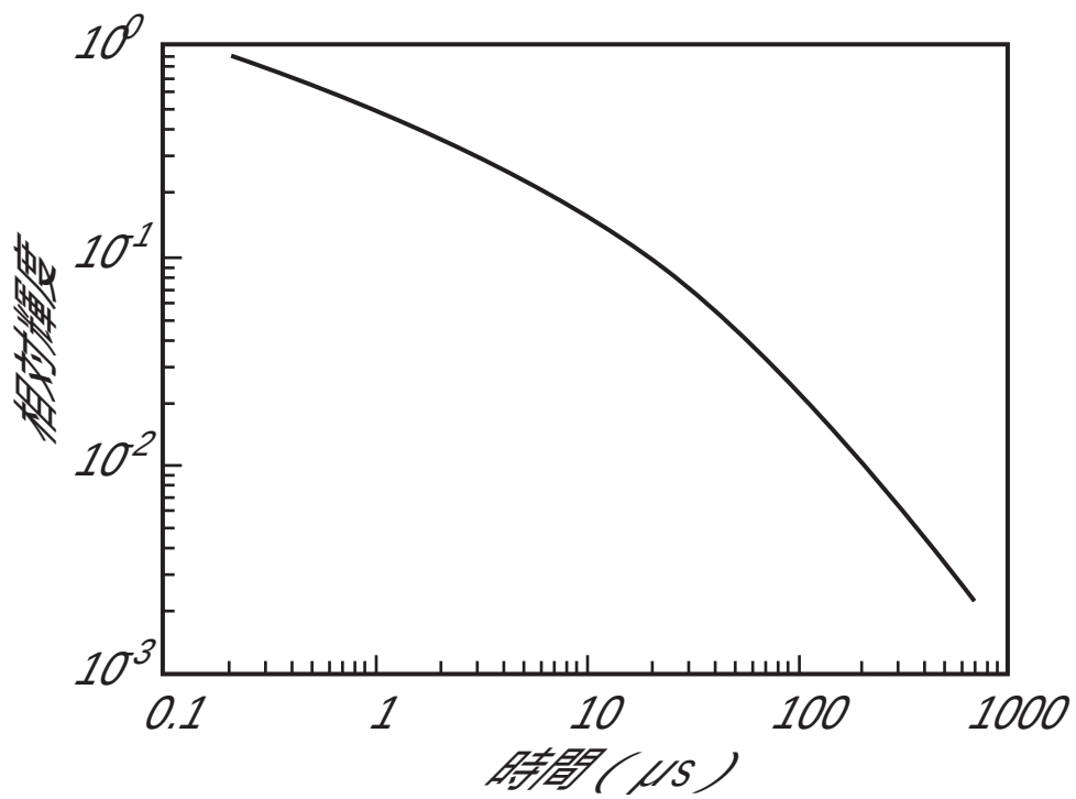
Figure 3.14: Lifetime of phosphor screen. X-axis is time ( \mu\text{sec.} ), Y-axis is relative brightness.
