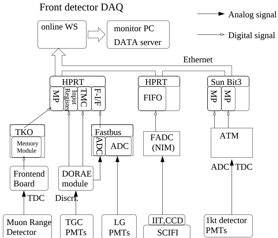
Figure 2.12: DAQ system of the near detector.
