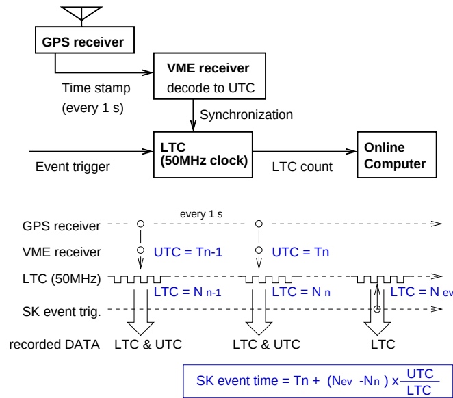
Figure 2.16: Overview of GPS system at SK. Block diagram (upper) and the timing chart (lower) are shown.
