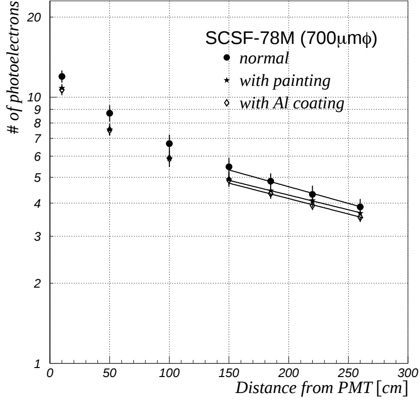
Figure 3.5: SciFi SCSF-78M attenuation measurement. The star and the white circle correspond to measurement with white paint and Al-coated fibers, respectively. An Al-coated fiber has a fitted attenuation length of 320cm.
