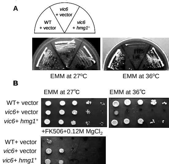
Figure3 Overexpression of the hmg1 + gene suppressed the temperature-sensitive phenotype of the vic6 mutant cells, but not its vic phenotype. (A) Expression of hmg1 + gene suppressed the temperature-sensitive phenotype of the vic6 mutant cells. Cells were streaked onto EMM plates and then incubated for 4 days at 27°C or 3 days at 36°C, respectively. (B) The hmg1 + gene failed to suppress the vic phenotype. Wild-type and vic6 mutant cells were dropped onto the plates as indicated and then incubated for 4 days at 27°C or 3 days at 36°C, respectively.
