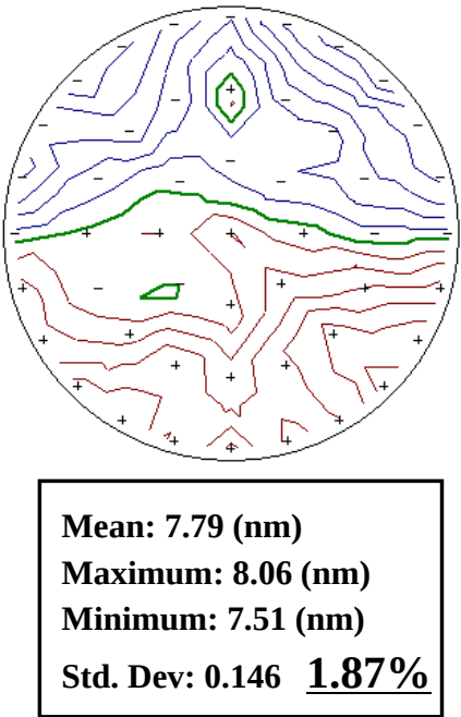
Fig. 2-16. Amorphized layer thickness uniformity map (121 point measured by SE) of a Si wafer after He+ PIII implantation with a bias power of 100W.
