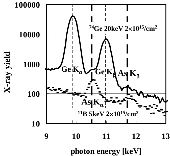
Fig. 3-9. PIXE spectra just after implantation with Ge (solid line) and with B (dashed line).
