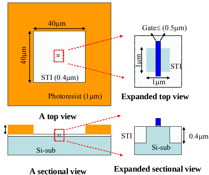
Fig. 4-16. A schematic of the transistor. The open area has a dimension of 1\text{ }\mu\text{m} \times 1\text{ }\mu\text{m} , and the most of the open area is occupied by the STI with a 400-nm depth.
