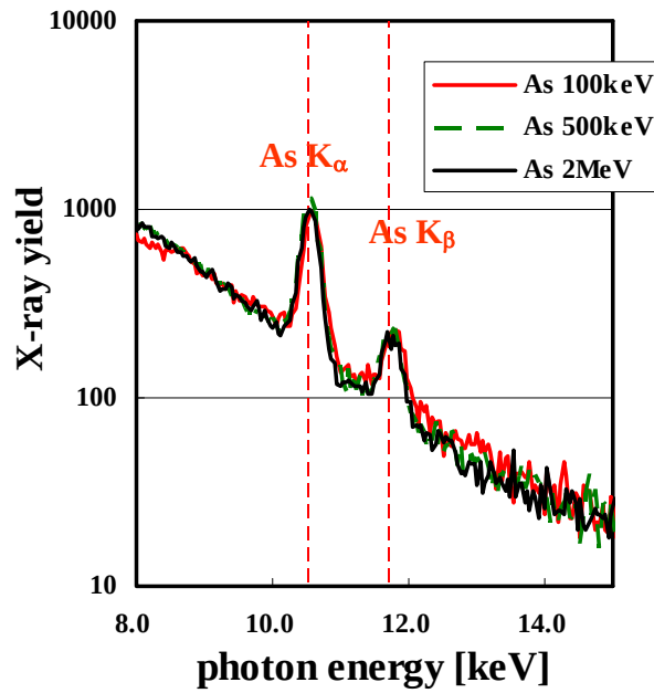
Fig. 3-8. PIXE spectra for 4.4 μm-thick photo-resist samples implanted with As ions, showing insensitivity to the ion energy.
