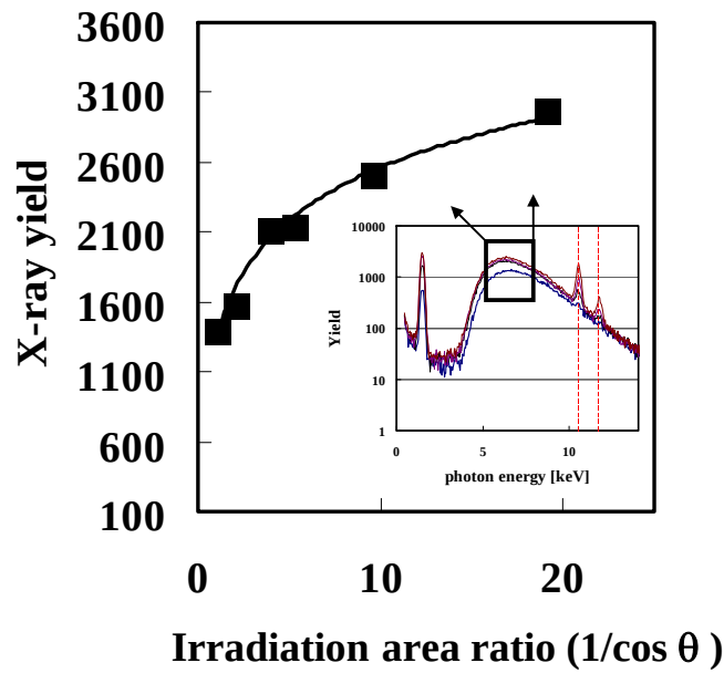
Fig. 3-4. Dependence of the peak height of bremsstrahlung continuum on irradiation area factor ( 1/\cos\theta ).
