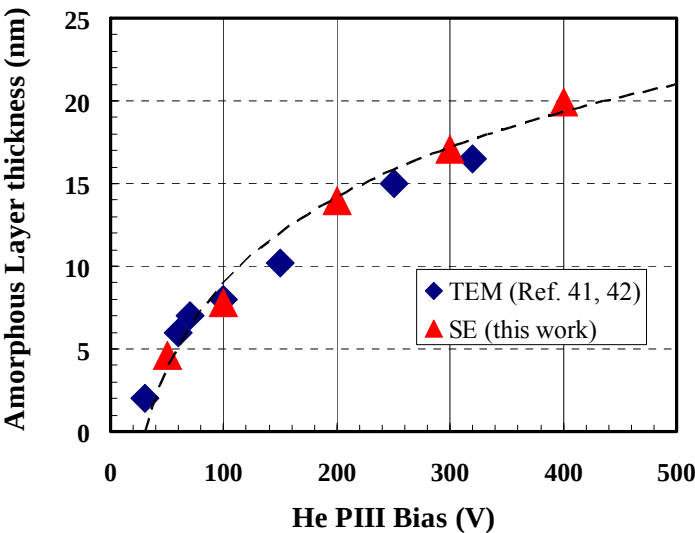
Fig. 2-15. Amorphized layer thickness of He+ PIII implanted wafers measured by TEM (Ref. 41, 42) and SE (this work) as a function of He PIII bias voltage.
