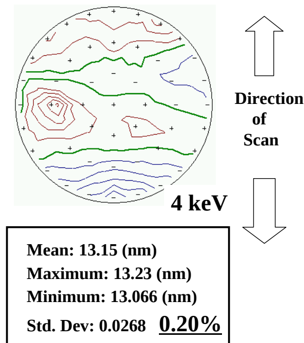
Fig. 2-14. Amorphized layer thickness uniformity map (49 point measured by SE) of a Si wafer after Ge implantation using a batch type ion implanter.
