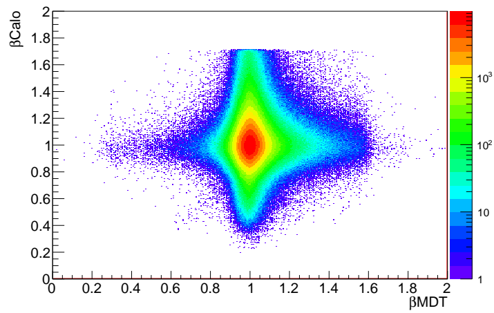
(b) \beta_{\text{MDT}} vs \beta_{\text{Calorimeter}}
