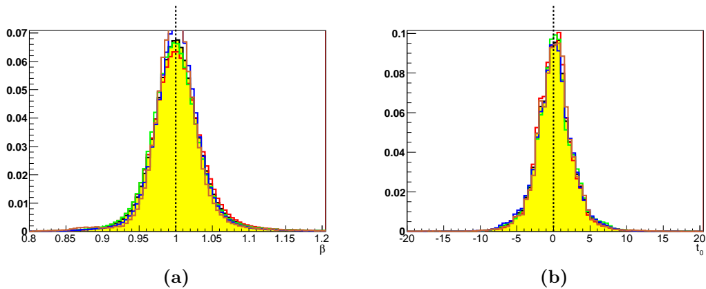
Figure A.10.: RPC (a) \beta (b) t_0 in 0.50 < |\eta| < 1.20 region (yellow). Overlaid lines are sub-distributions for 0.5 < |\eta| < 0.68 < |\eta| < 0.85 < |\eta| < 1.03 < |\eta| < 1.20 .
