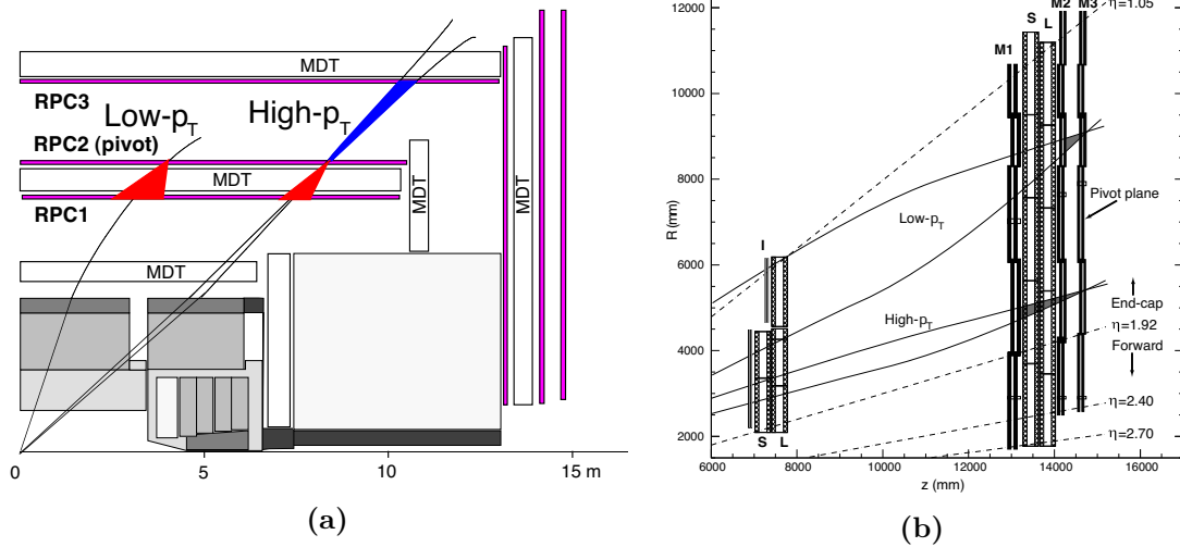
Figure 3.23.: The single muon trigger
