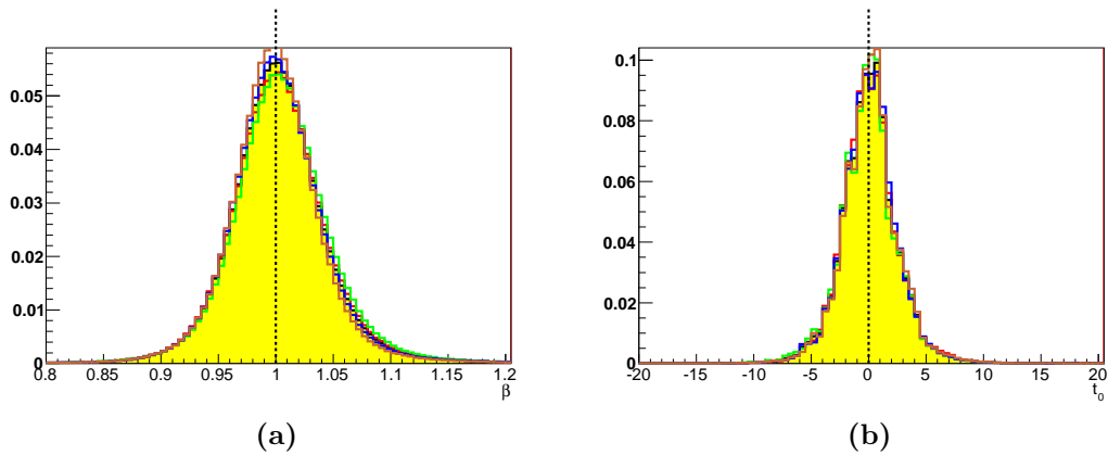
Figure A.9.: RPC (a) \beta (b) t_0 in 0.10 < |\eta| < 0.50 region (yellow). Overlaid lines are sub-distributions for 0.1 < |\eta| < 0.2 < |\eta| < 0.3 < |\eta| < 0.4 < |\eta| < 0.5 .
