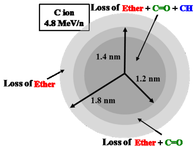
Fig. 4.3.1. Layered structure of C ion with an energy of 4.8 MeV/u.
