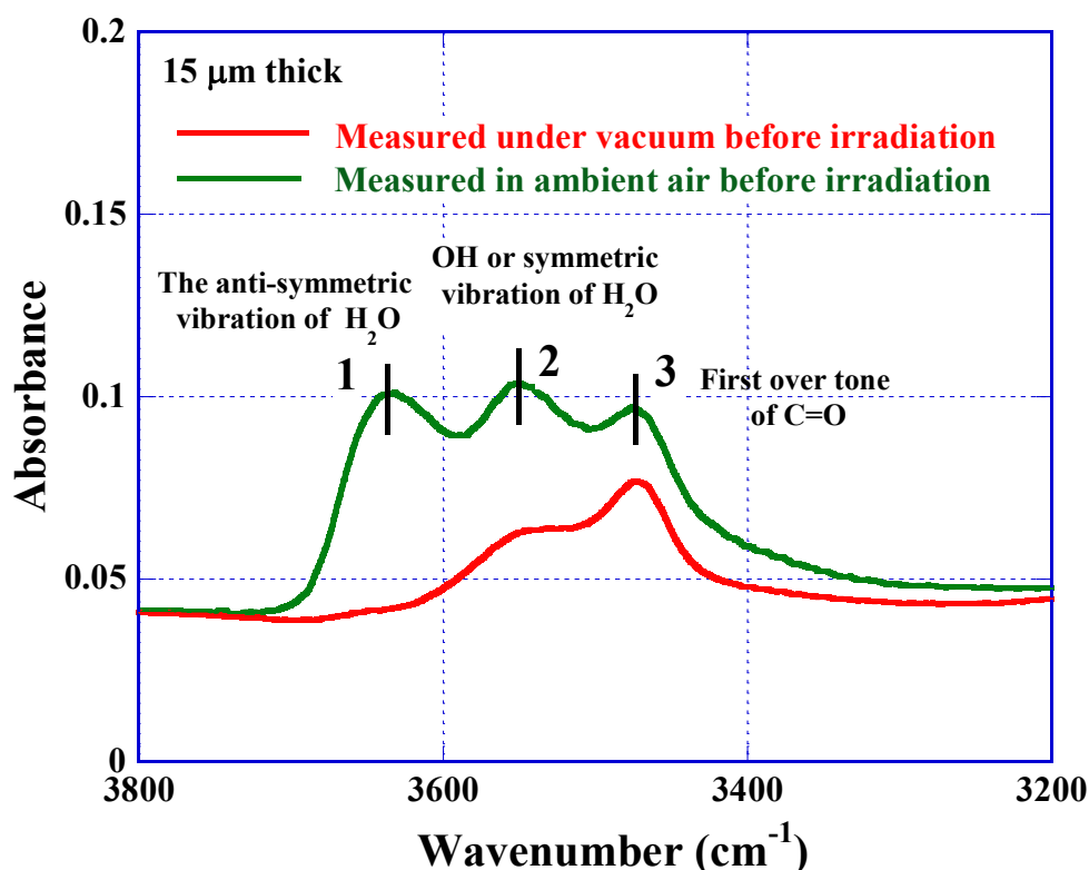
Fig. 3.2.1. IR spectra of pristine PADC film with a thickness of 15 \mu\text{m} measured in ambient air (green) and under vacuum (red).
