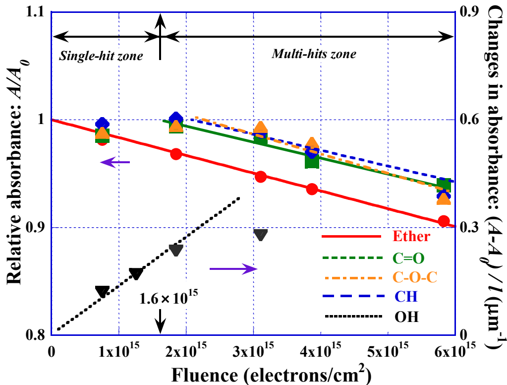
Fig. 4.2.1. Reduction of the relative absorbance of ether, carbonyl, C-O-C and CH groups (left axis) and increase of the absorbance around OH groups (right axis) against the fluence (Kusumoto et al., 2016b).
