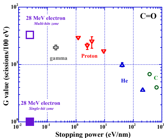
Fig. 4.2.6. G values for loss of carbonyl against the stopping power (Kusumoto et al., 2016b). The deposited energy per unit distance and average LET in water are adopted in the cases of 28 MeV electron and gamma ray, respectively.
