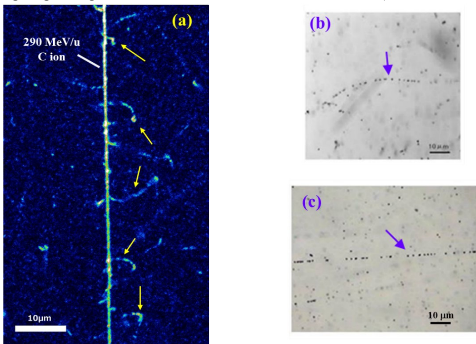
Fig. 1.1.5. An example of (a) fluorescence image after the irradiation with C ion with an energy of 290 MeV/u and images of Nuclear Emulsion after the exposure to (b) a 1 MeV electron and (c) a 100 MeV electron track (Fukuda et al., 2010).
