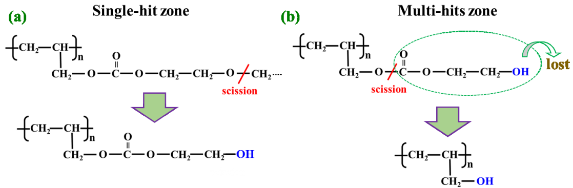
Fig. 4.2.4. Two steps damage formation process in PADAC. The ether is broken in Single-hit zone (a) and carbonate ester is lost with the OH groups in Multi-hits zone (b).
