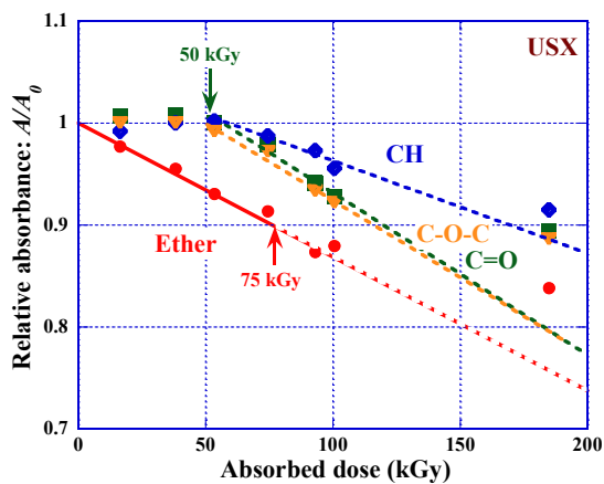
Fig. 4.1.3. Reduction of the relative absorbance of ether, carbonyl, C-O-C and CH groups in PADC irradiated with USX.
