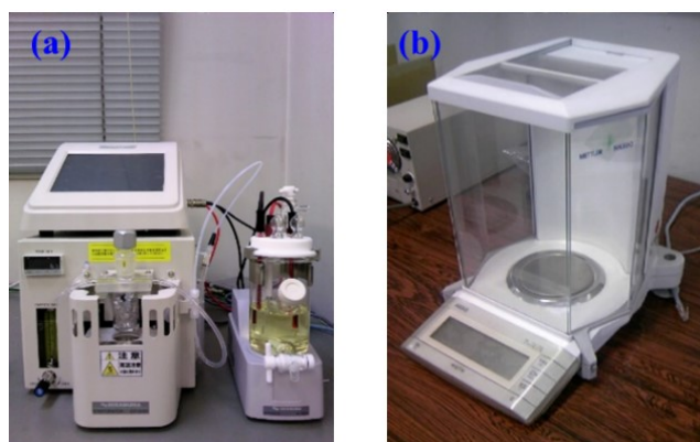
Fig. 2.3.1. Karl Fischer Coulometric Titrator, EV-200 (a), and electronic balance, AG245 (b),.
