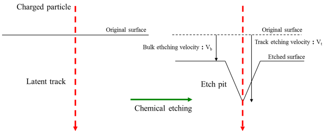
Fig. 1.1.1. A latent track and an etch pit.
