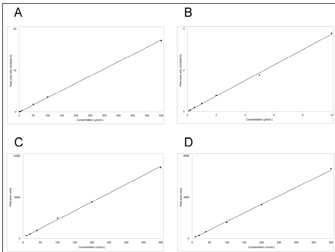
Figure S2. Calibration curves of squalene ( r=0.9997 , A), lanosterol ( r=0.9992 , B), FPP ( r=0.9992 , C), and GGPP ( r=0.9993 , D)
