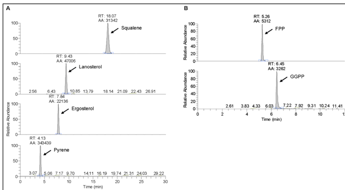
Figure S1. LC-MS/MS analysis of isoprenoids. A) SRM chromatograms of squalene, lanosterol, ergosterol, and pyrene in the standard solution. B) SRM chromatograms of FPP and GGPP in the standard solution.
