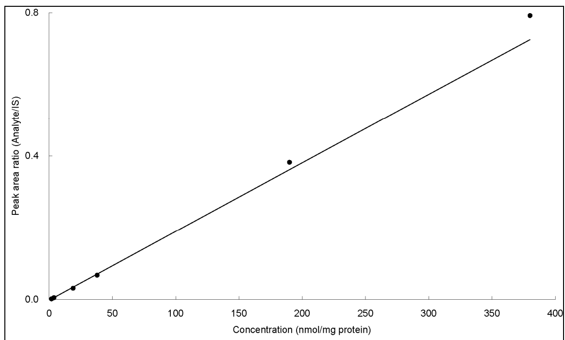
Figure S4. Calibration curve of ergosterol ( r=0.9967 )
