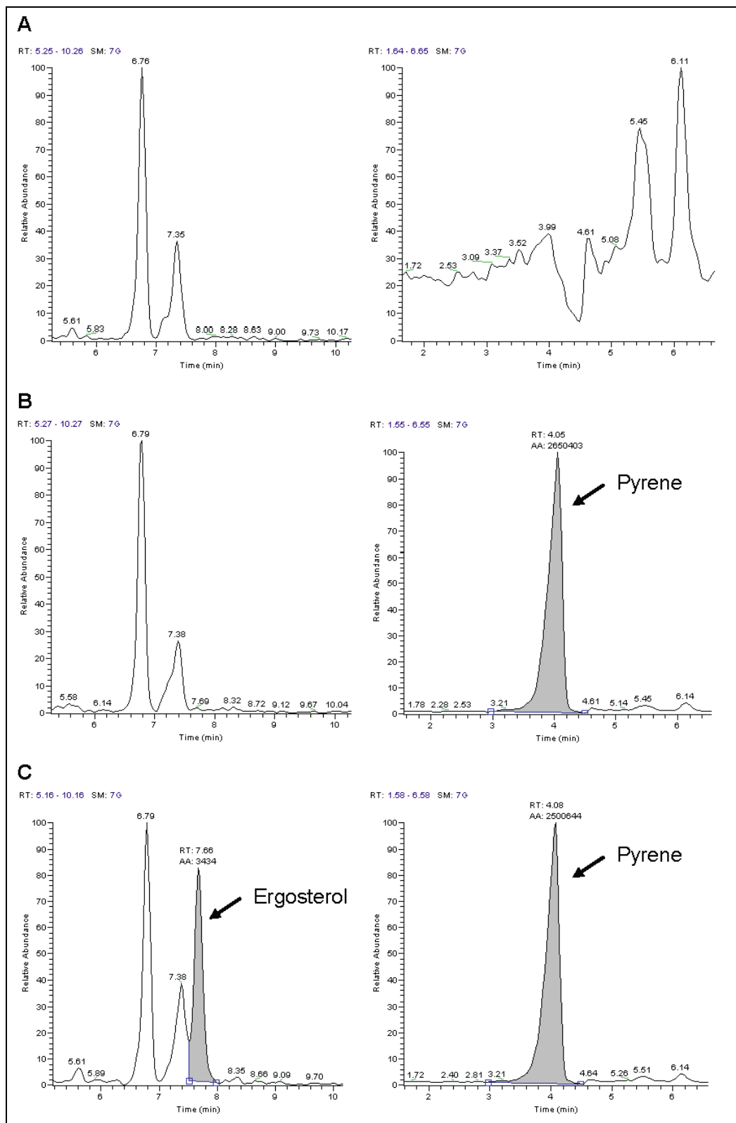
Figure S3. LC-MS/MS analysis of ergosterol in fission yeast extracts. SRM chromatograms of ergosterol (Left) and pyrene (Right) in the blank sample (A), the zero sample (B), and the LLOQ sample (C).
