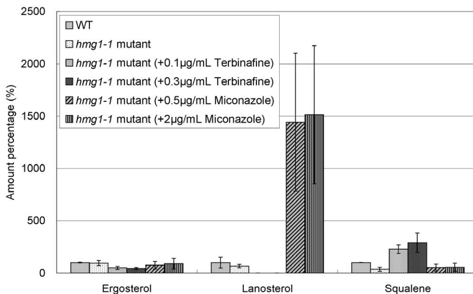
Figure 6. Effect of terbinafine and miconazole treatment on levels of ergosterol, lanosterol, and squalene in hmg1-1 mutant. Wild-type cells and hmg1-1 mutants were grown to saturation at 27°C in liquid YPD medium. Cells were further incubated at 27°C for 10 h in the absence or presence of terbinafine (0.1, 0.3 µg/ml) or miconazole (0.5, 2.0 µg/ml) as indicated, and then ergosterol, lanosterol, and squalene of the strains were extracted and determined. Error bars represent standard deviations (n = 3 experiments). doi:10.1371/journal.pone.0049004.g006
