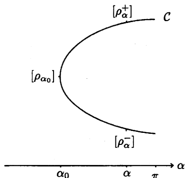
Fig. 1 : The curve \mathcal{C} from Proposition 3.1.
