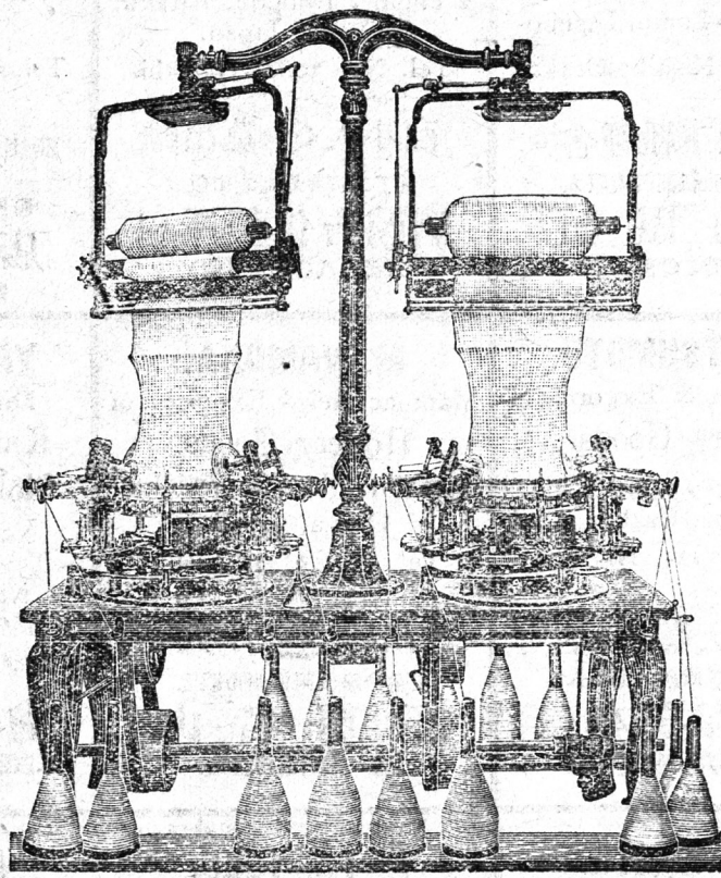
械機織上捲スヤリメ式木鈴
